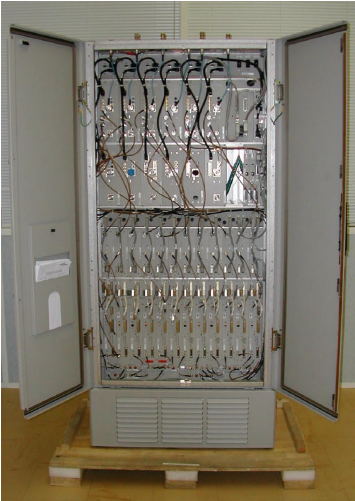
Figure 2 – S12000 Indoor Front View with Doors Open
