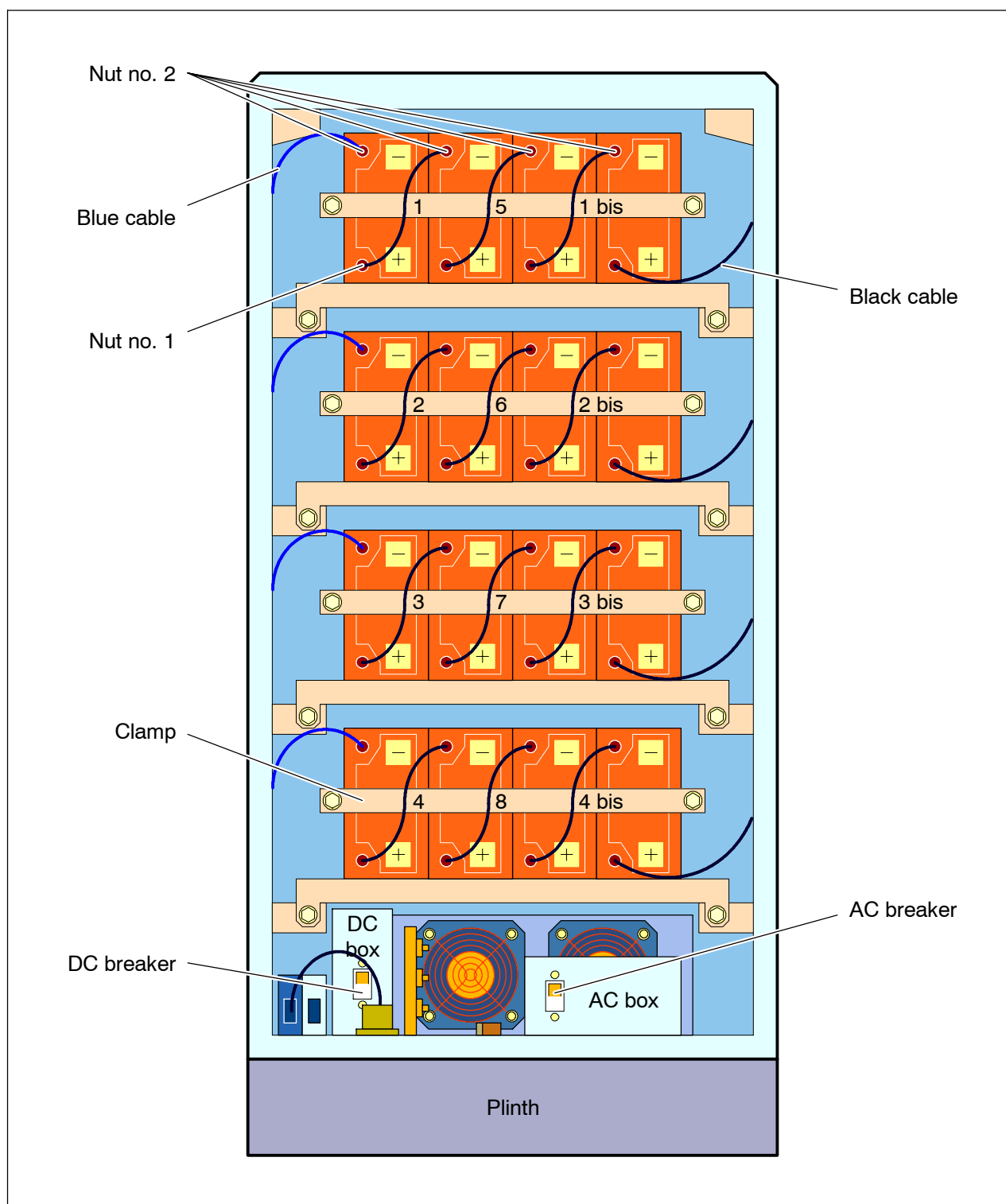
Figure 1-3 External battery cabinet of the S12000 Outdoor BTS (SBS 60 batteries)
