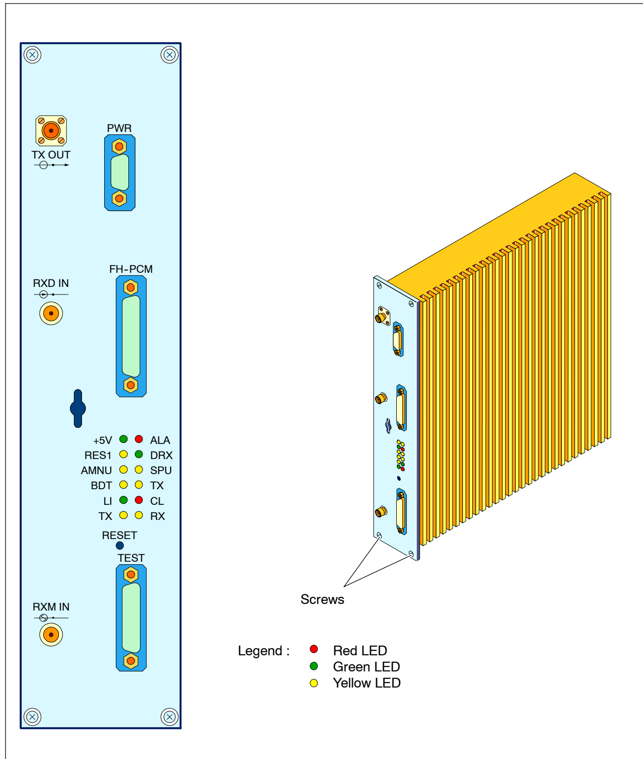
Figure 2-24 DRX module
