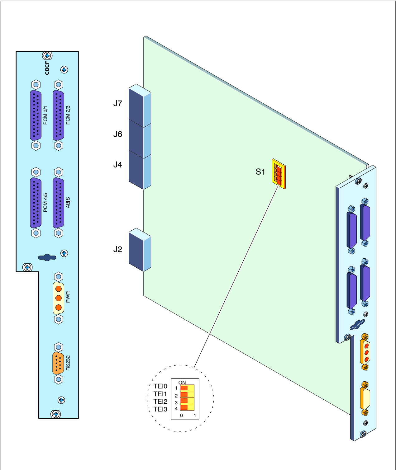
Figure 2-22 BCFICO board
