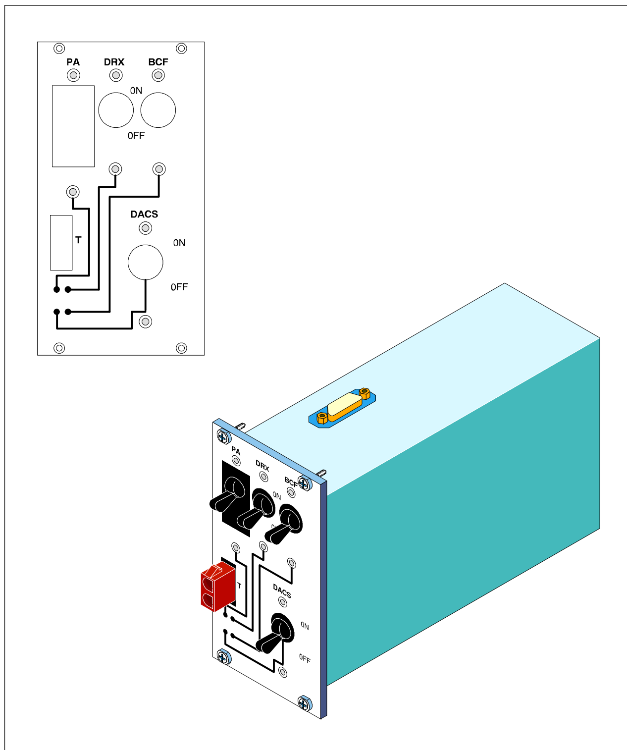
Figure 2-32 DCU module
