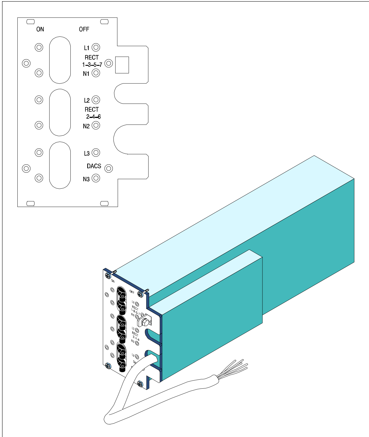
Figure 2-33 ADU module
