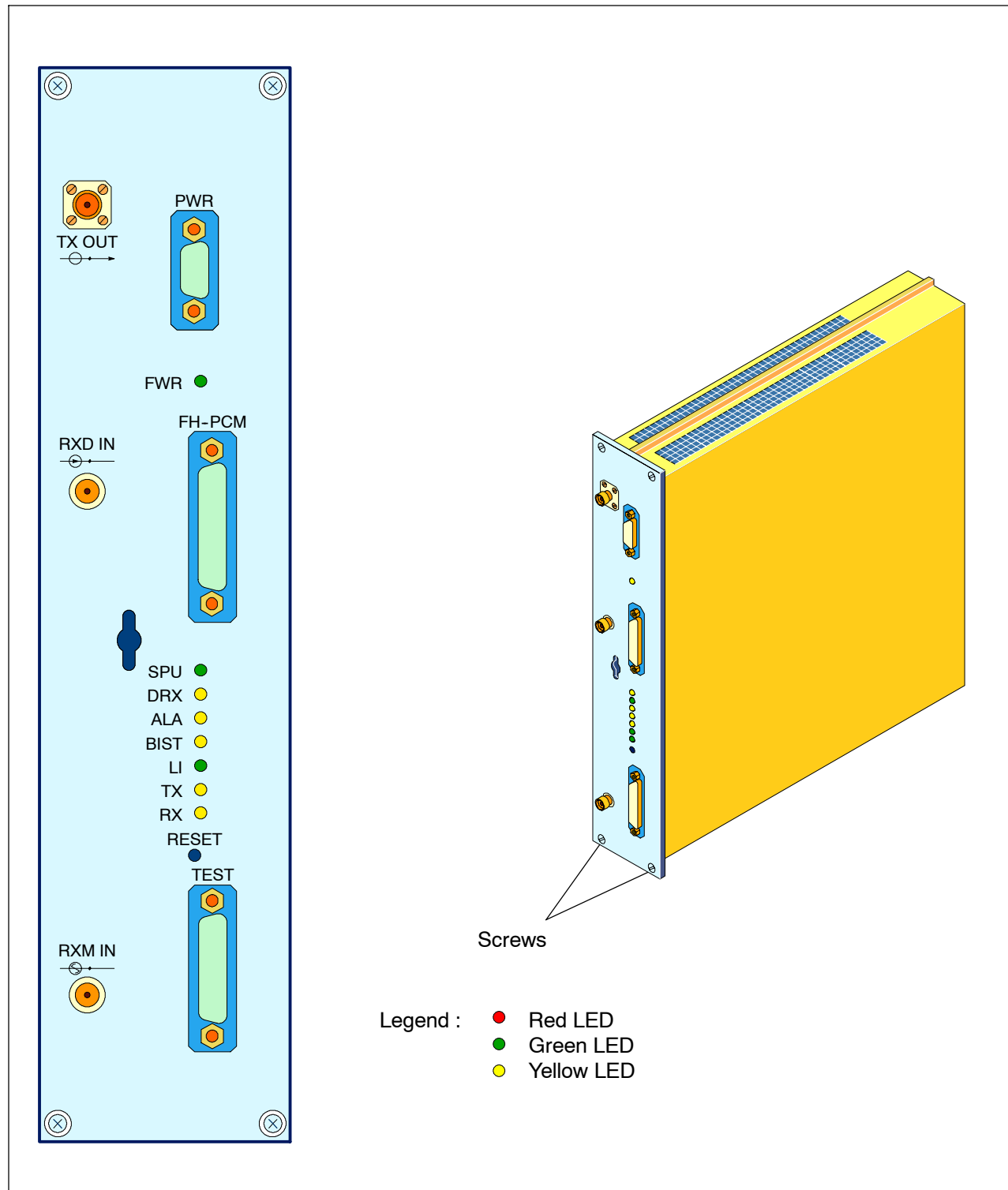
Figure 2-25 e-DRX module
