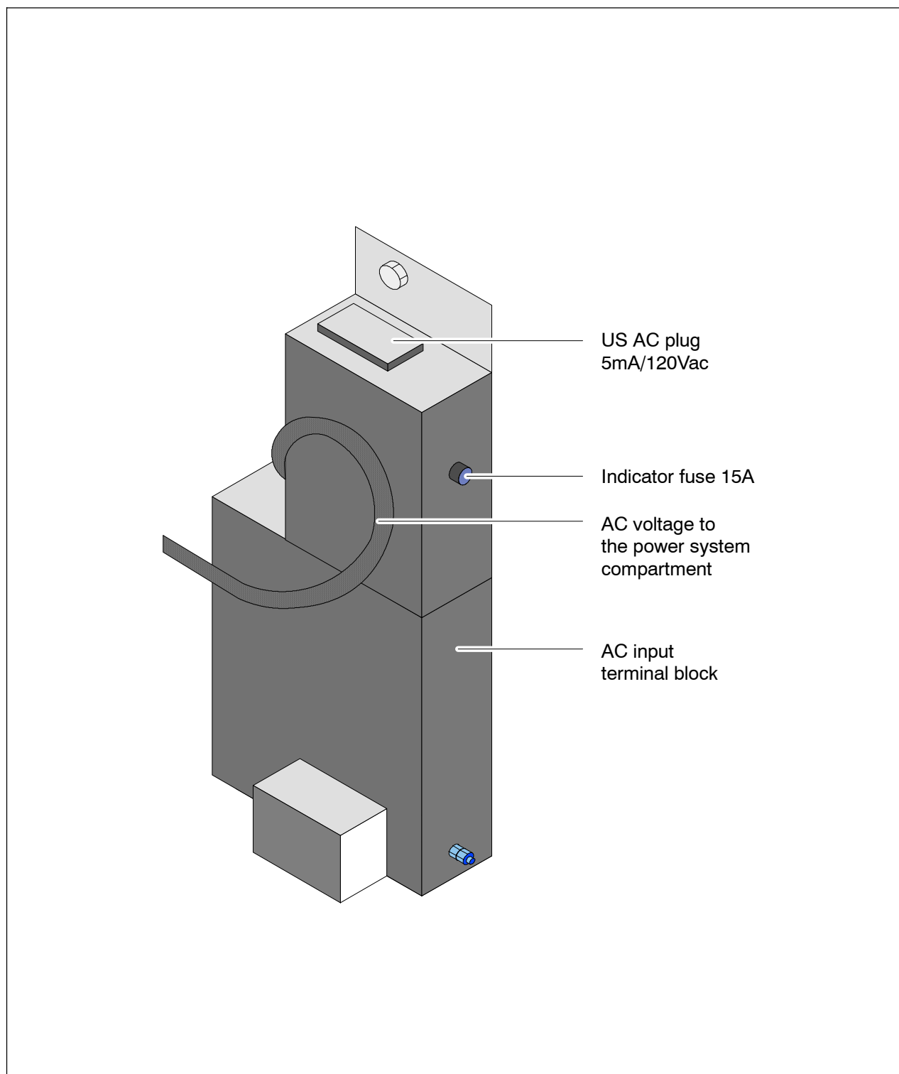
Figure 1-12 AC box/GIPS with US type user AC plug BTS
