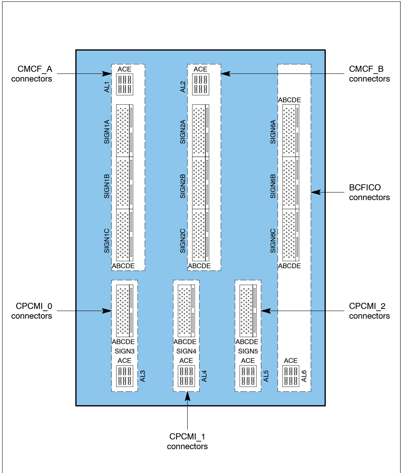
Figure 2-23 CBP board
