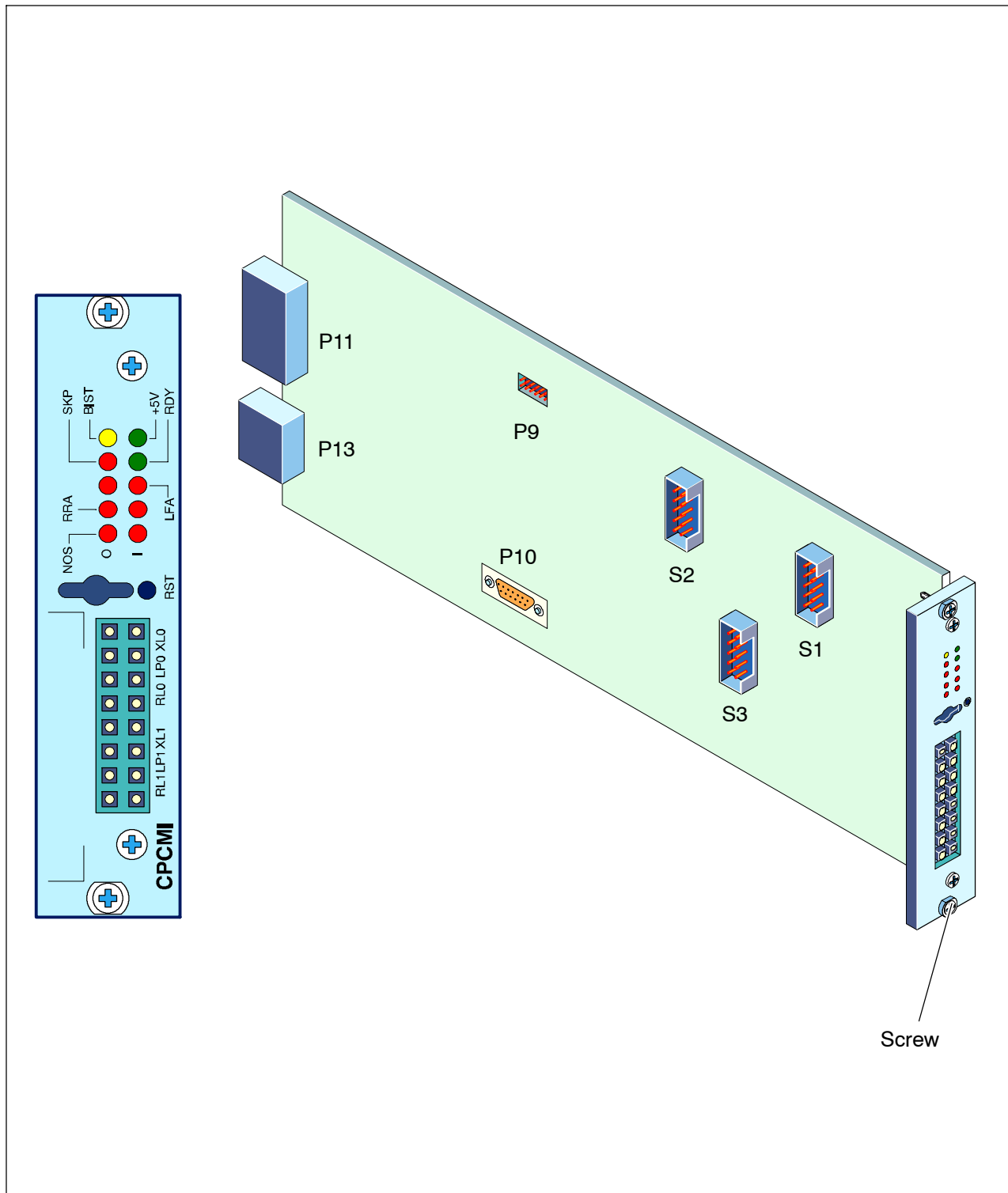
Figure 2-19 CPCMI board
