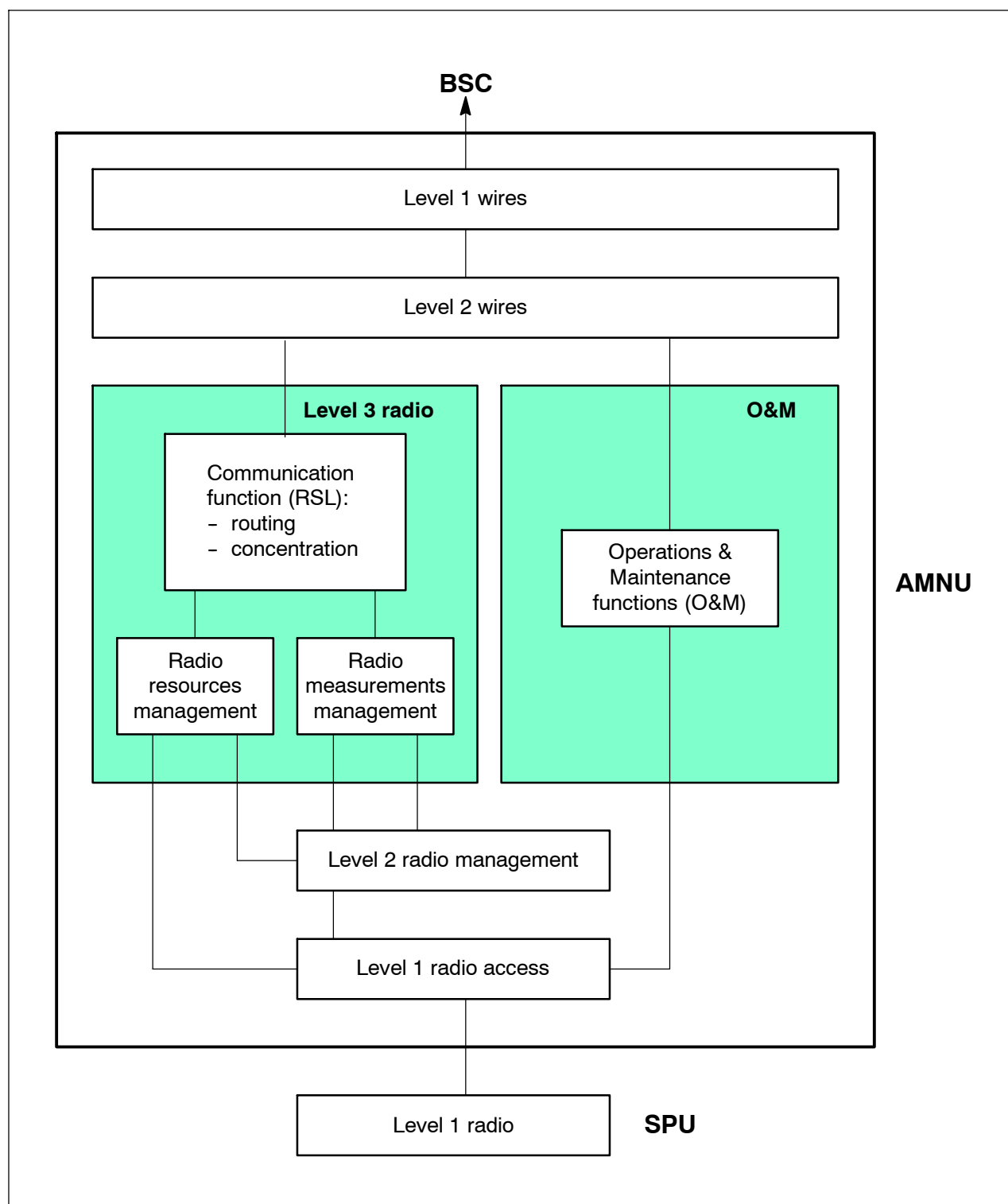
Figure 3-5 AMNU functions
