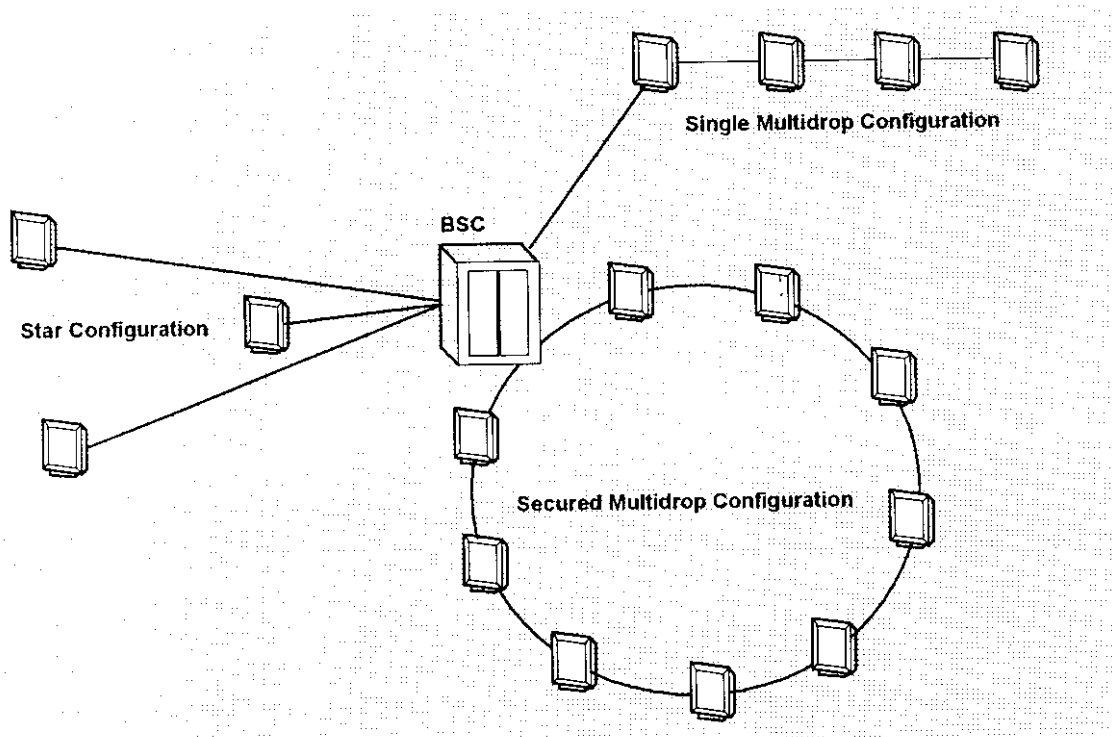
Figure 3: S2000L BTS connections to the BSC
