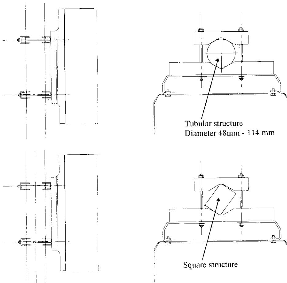
Figure 27 - Pole mounting
