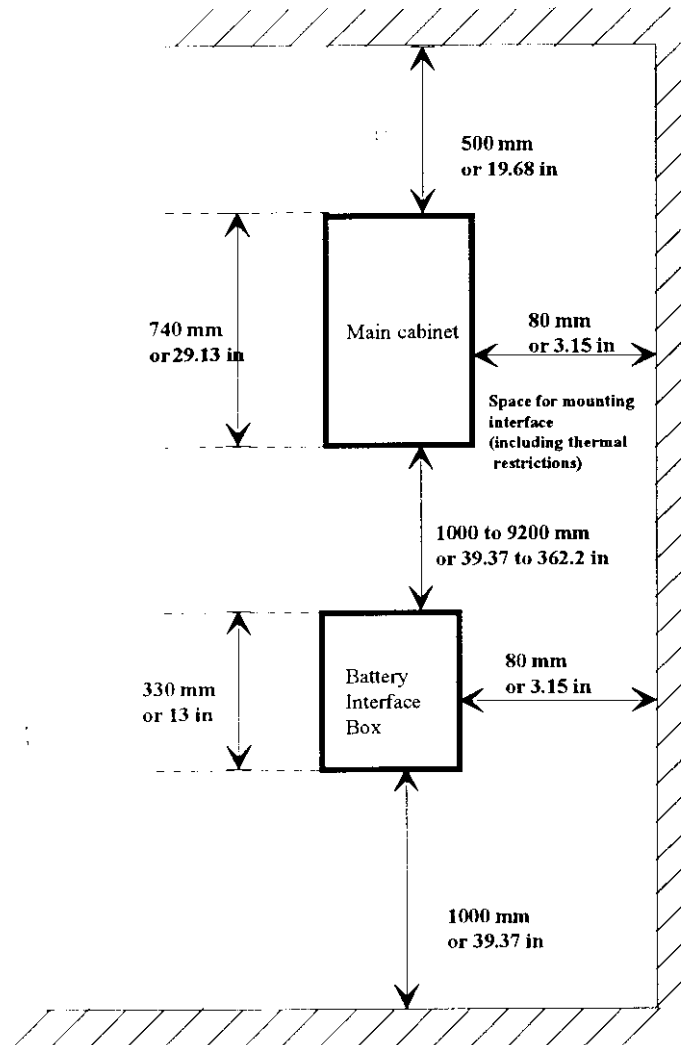
Figure 3 - Base unit and battery interface box clearance (side view)
