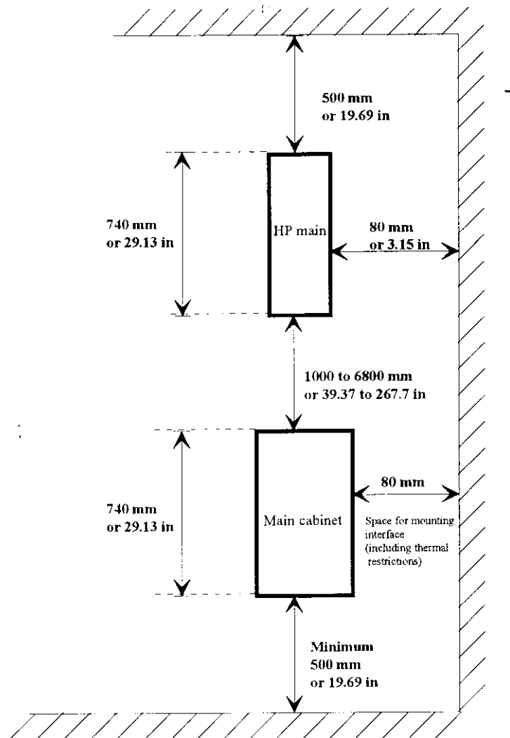
Figure 4 - Base unit and HPRF clearance (side view)
