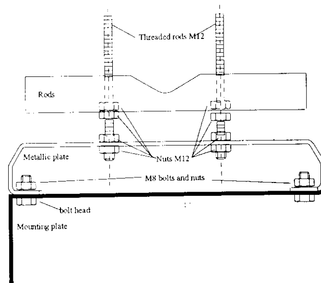
Figure 26 - Mounting kit with tilt adjustment
