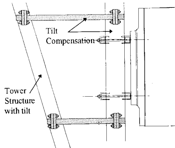
Figure 28 - Tower mounting
