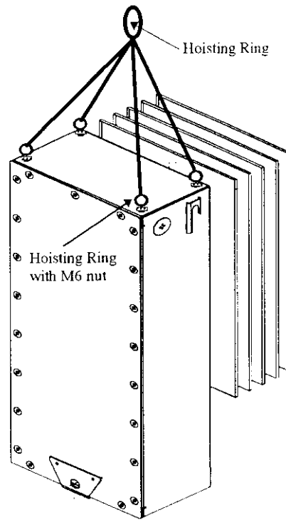
Figure 34 - HPRF hoisting
