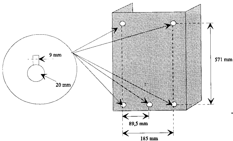
Figure 15 - HPRF mounting plate
