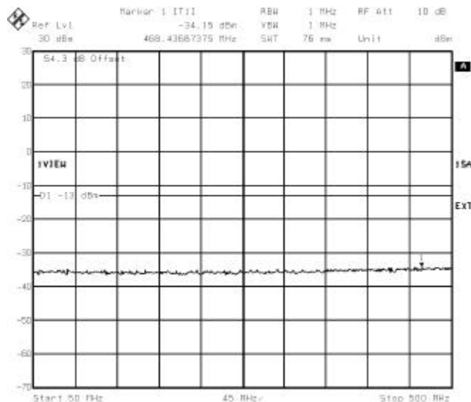
Figure 12: 50 MHz – 500 MHz
