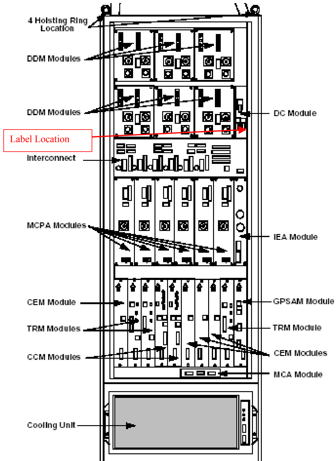
Picture 2: FCC Label Location
