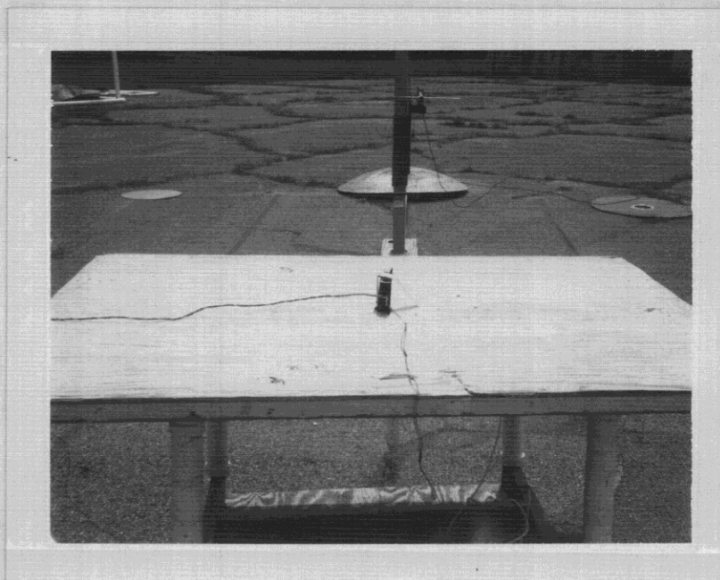
Figure 5.4. DUT on the open-site test table showing the worst case position and orientation with respect to the measuring antenna at "fundamental".
