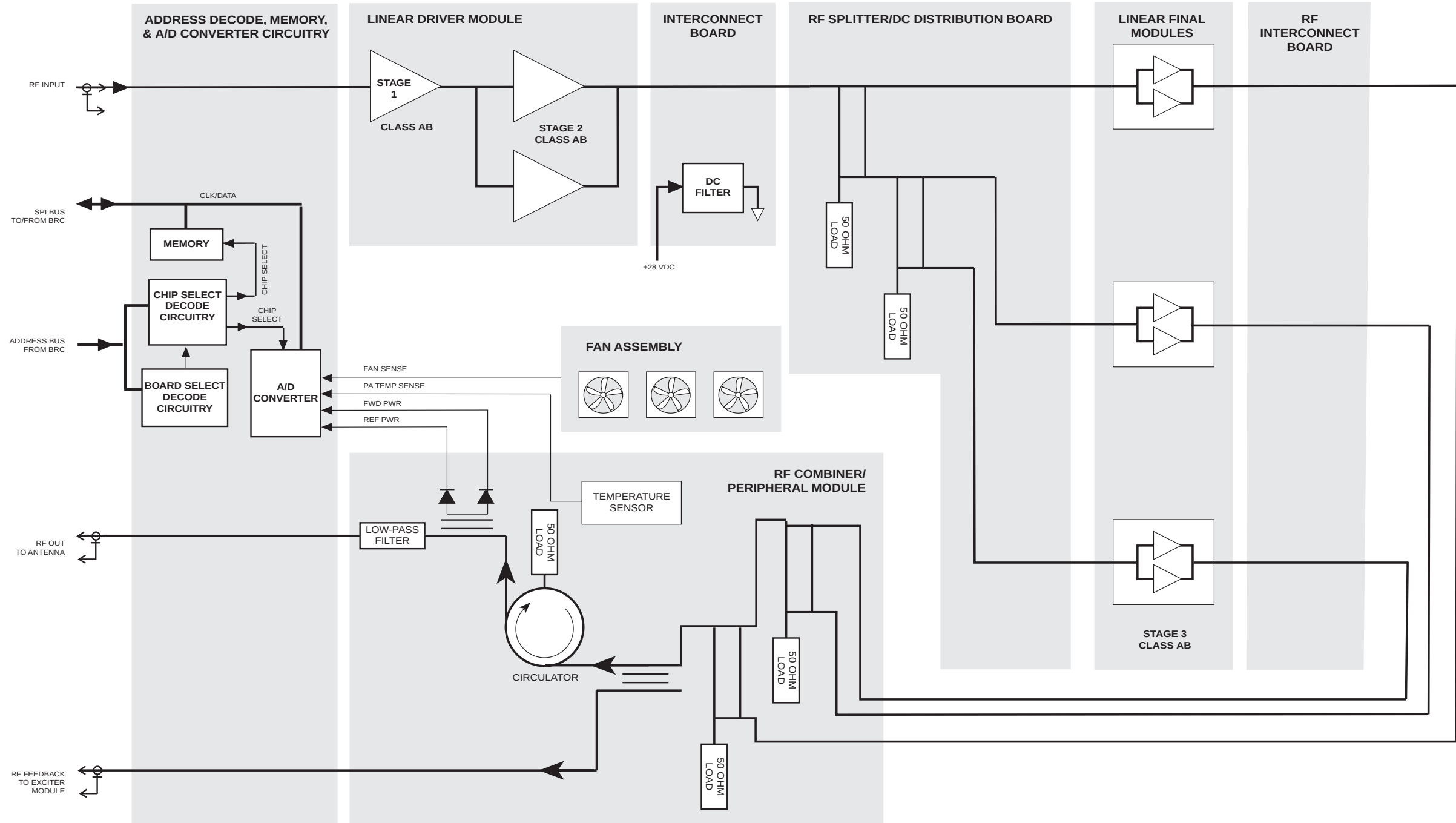
Figure 5 TLF2020 (CLF1772) 40W- 800 MHz PA Functional Block Diagram (Sheet 1 of 1)
