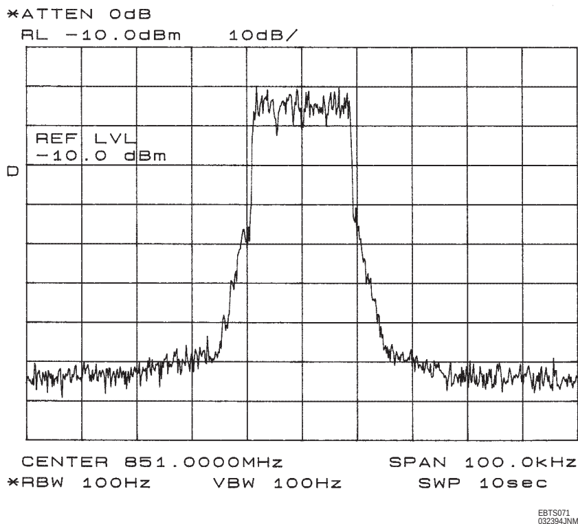
Figure 3 Generation 2 Carrier Spectrum
