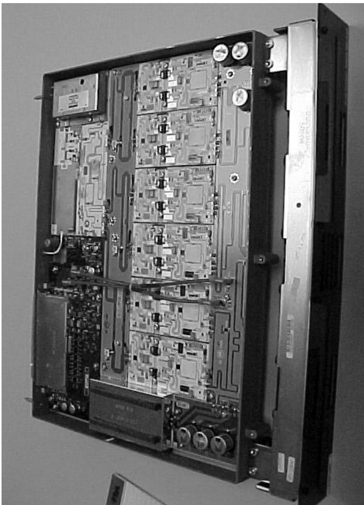
Power Amplifier Module, Top View, Shields Removed
