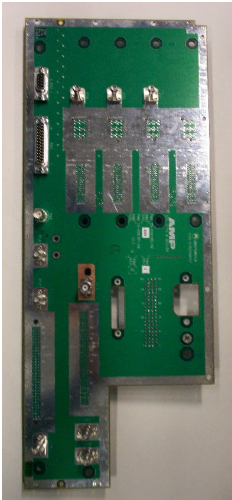
Backplane Board, Back Side
