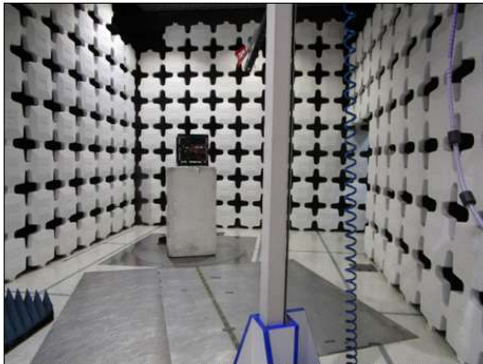
Test Setup for Case Spurious Radiated Emissions, Above 1GHz – Antenna Polarization Horizontal
