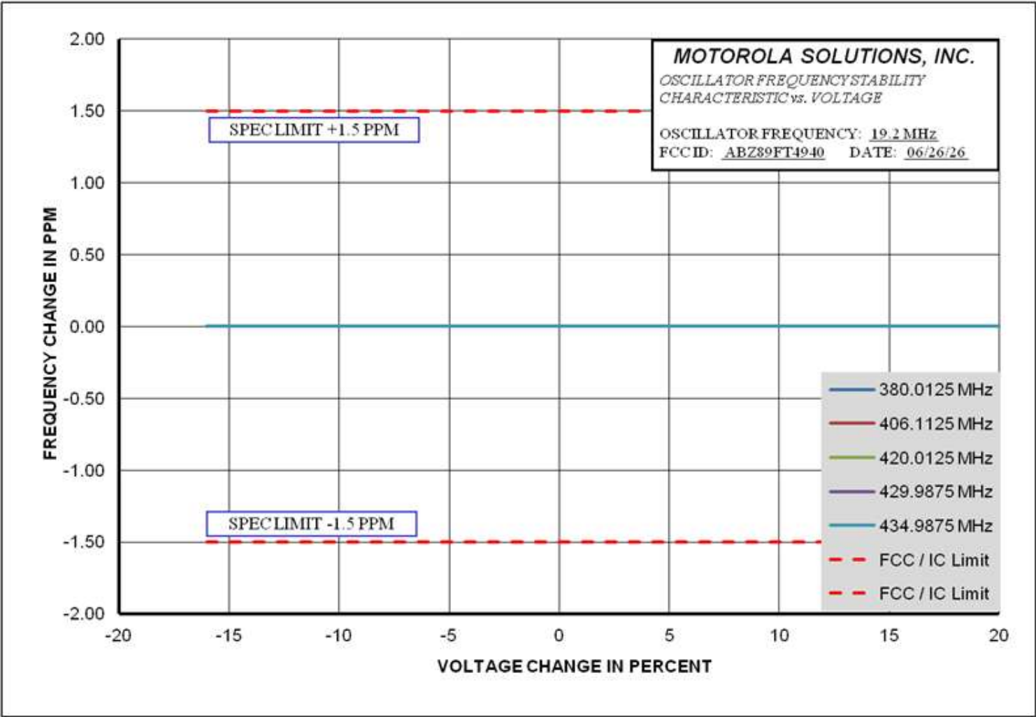
Frequency Stability Vs Voltage
