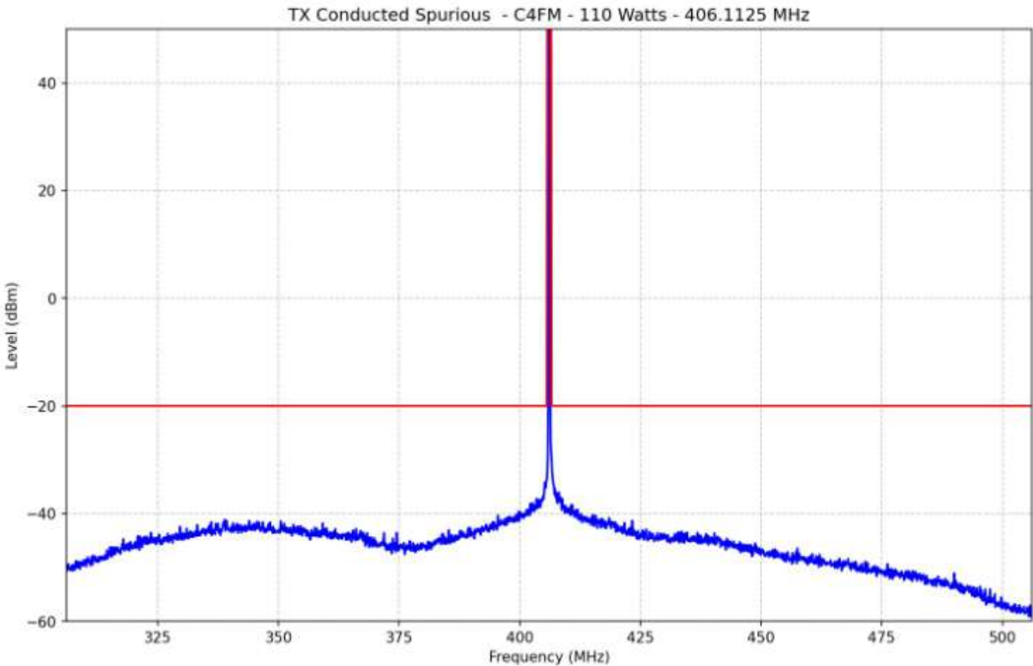
Conducted Spurious Emission Spectrum – 110 Watts C4FM – 200 MHz Span
