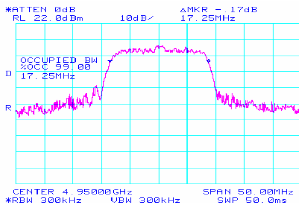
Plot 17. Measured Occupied Bandwidth
