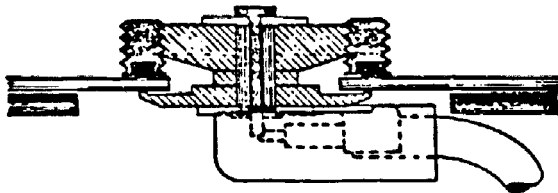
Figure 7. Double Roof (with Dome Light) Installation
