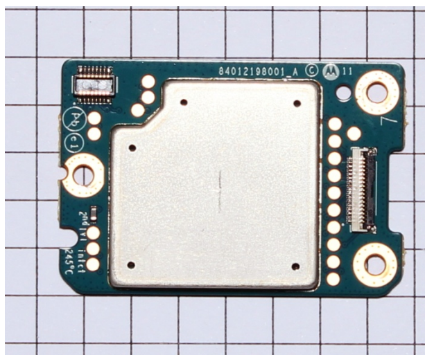
GOB board with Shield (Bottom)
