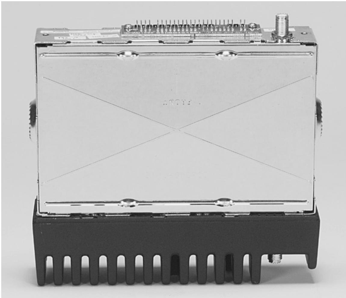
TRANSCEIVER TOP VIEW WITHOUT COVER
