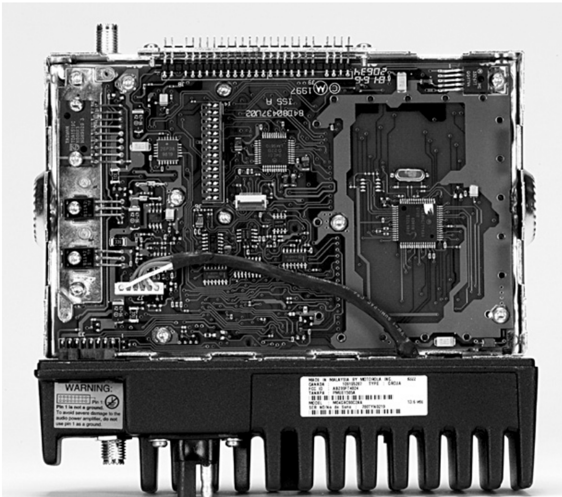
TRANSCEIVER BOTTOM VIEW WITHOUT COVER AND SHIELD
