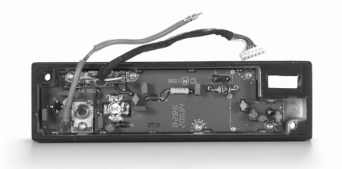
RF PA FRONT VIEW WITHOUT SHIELD
