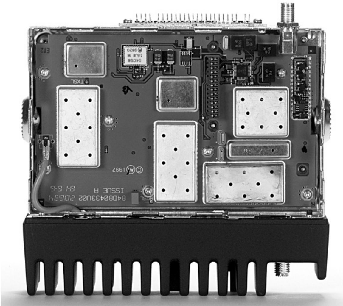
TRANSCEIVER TOP VIEW WITHOUT COVER AND SHIELD
