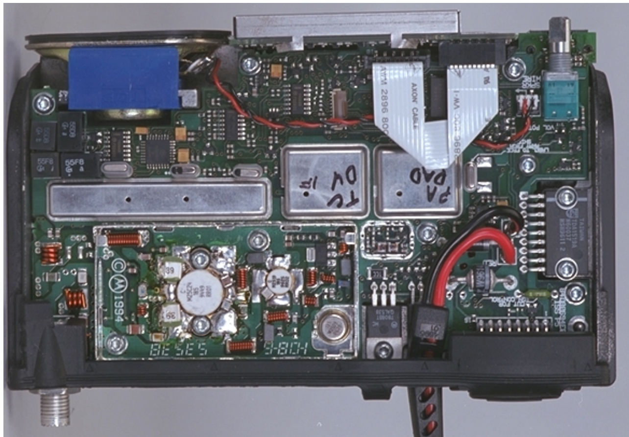
TOP VIEW (Cover and PA shield removed)
