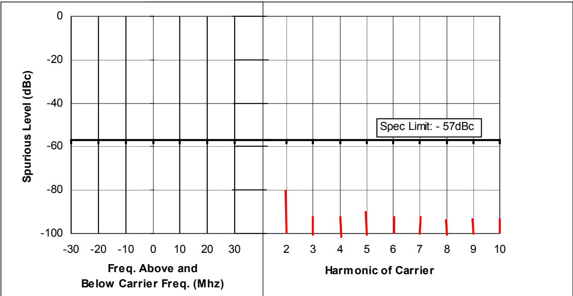
Figure 6F-10: 25 Watts, 438.0125 MHz, 25 kHz Channel Spacing
