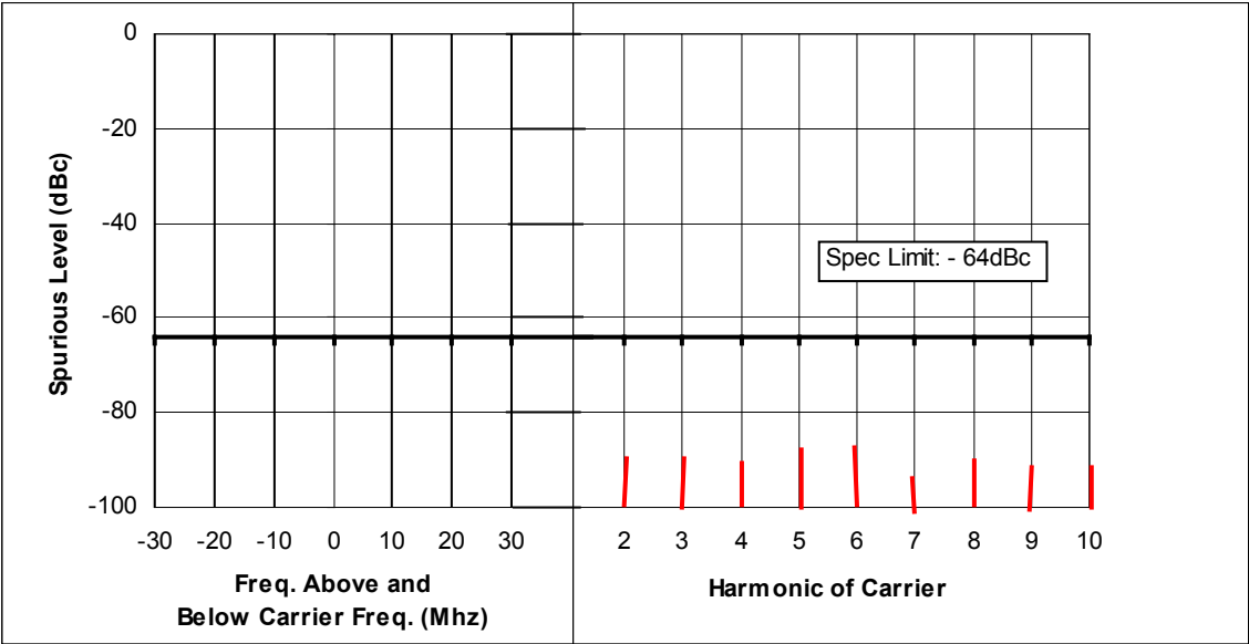
Figure 6F-9: 25 Watts, 469.9875 MHz, 12.5 kHz Channel Spacing
