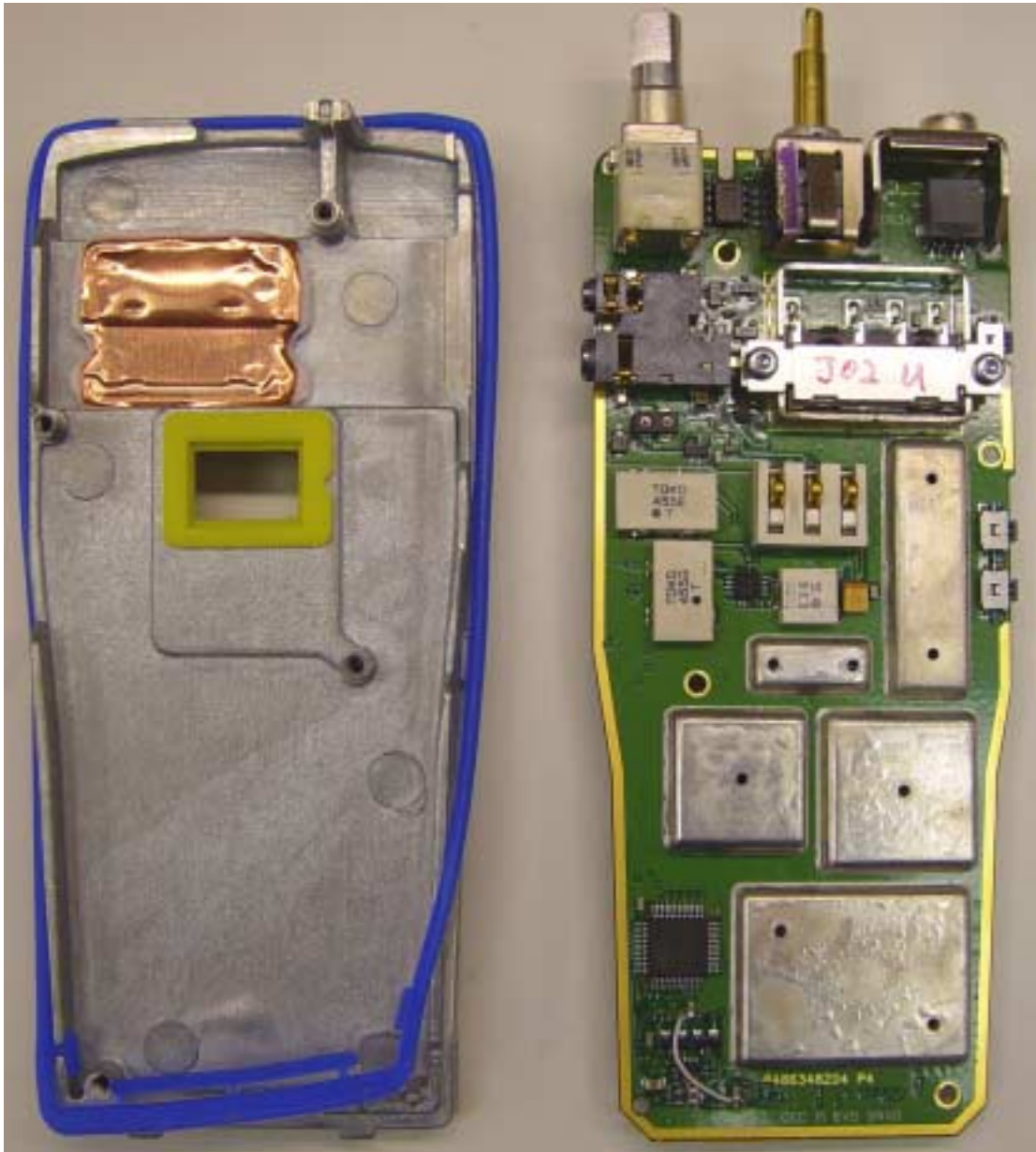
VIEW OF CIRCUIT BOARD REMOVED FROM CHASSIS (MATING SURFACES OF CIRCUIT BOARD AND CHASSIS ARE SHOWN)
