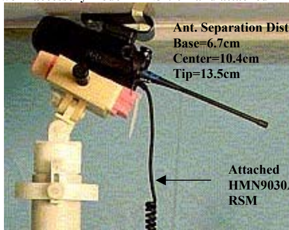
Figure 3: Assessment @ the Abdomen; DUT w/ body worn accessory model RLN5496A and attached HMN9030A RSM
