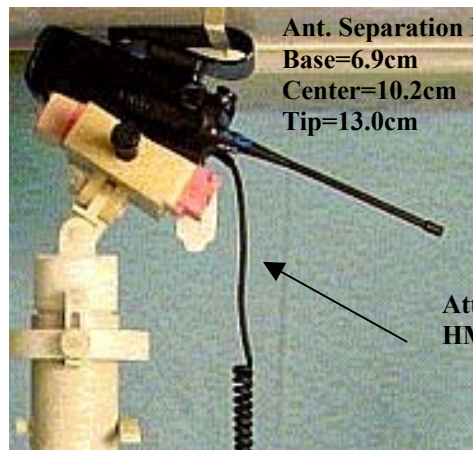
Figure 4: Assessment @ the Abdomen; DUT w/ Body worn accessory model RLN5497A and attached HMN9030A RSM
