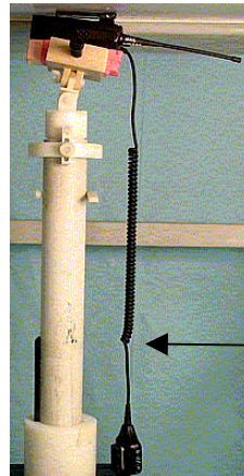
Figure 2. Assessment @ the Abdomen; DUT w/ body worn accessory model HLN8255 and attached HMN9030A RSM (Same position used w/ antenna adaptor attached)
