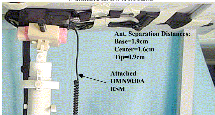
Figure 6: Assessment @ the Abdomen; DUT w/ body worn accessory model HLN6602A W/ attached HMN9030A RSM.
