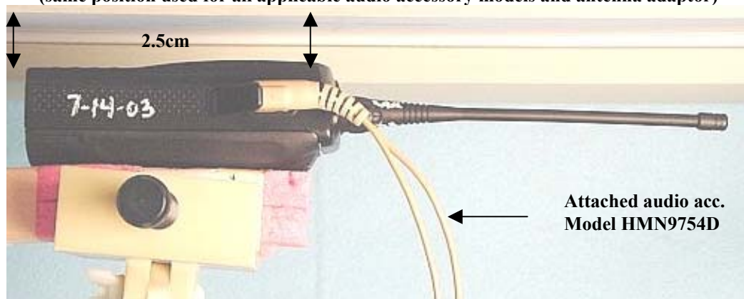
Figure 8: Assessment @ the Face; DUT front w/ 2.5cm separation With attached Audio accessory model HMN9754D (same position used for all applicable audio accessory models and antenna adaptor)
