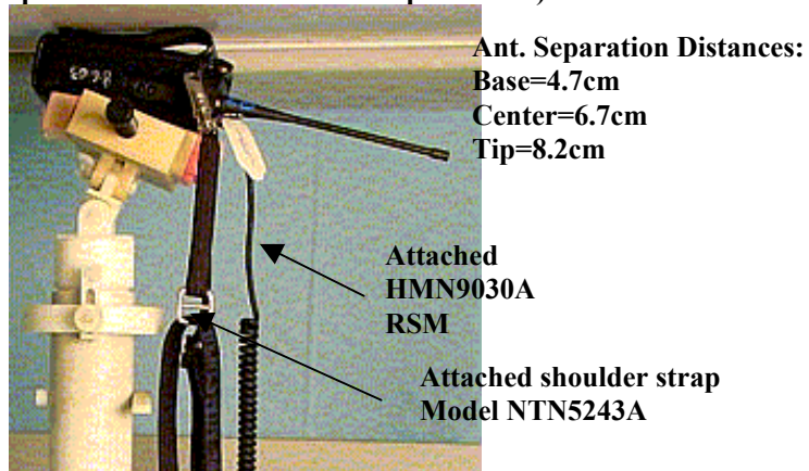
Figure 5: Assessment @ the Abdomen; DUT front w/ body worn accessory model RLN5498A W/ attached HMN9030A RSM and shoulder strap model NTN5243A (Same position used w/o shoulder strap attached)
