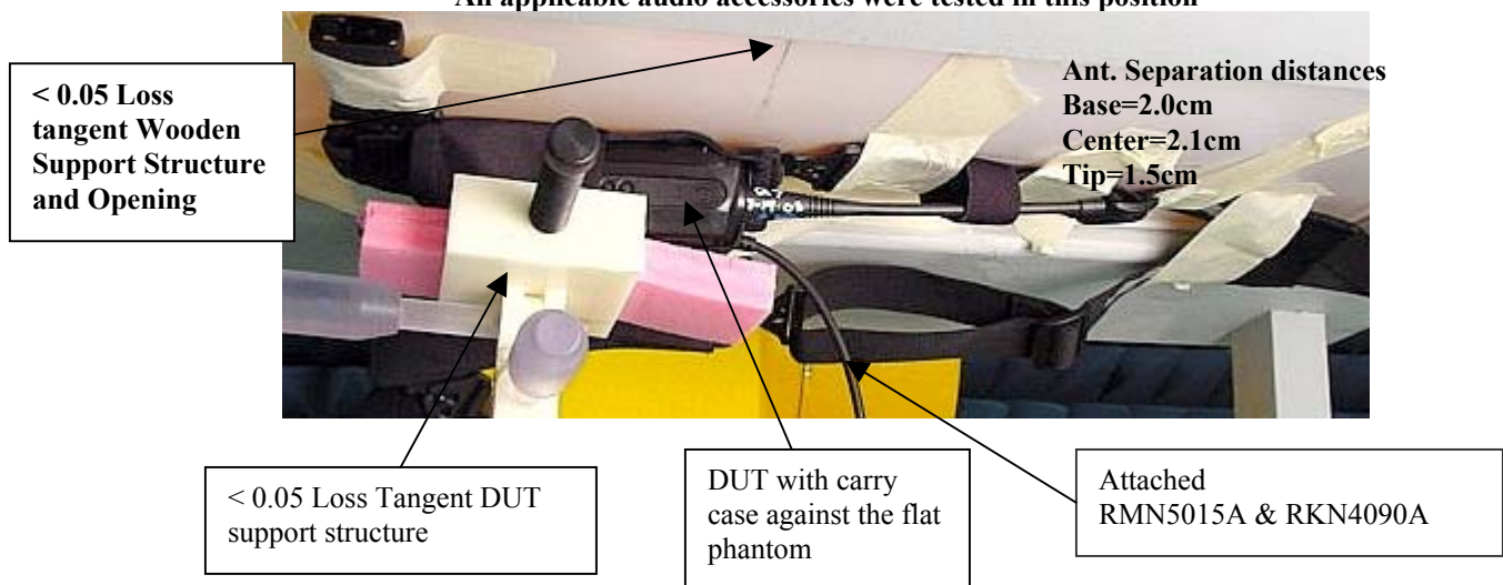
Figure 1: Highest S.A.R. Test Position at the abdomen (DUT w/ carry case model RLN4570A against the flat phantom w/ attached audio accessory model RMN5015A & RKN4090A) All applicable audio accessories were tested in this position
