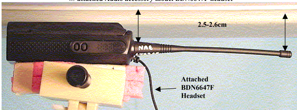
Figure 7: Assessment @ the Abdomen; DUT w/ back/antenna separated 2.5cm w/ attached Audio accessory model BDN6647F headset
