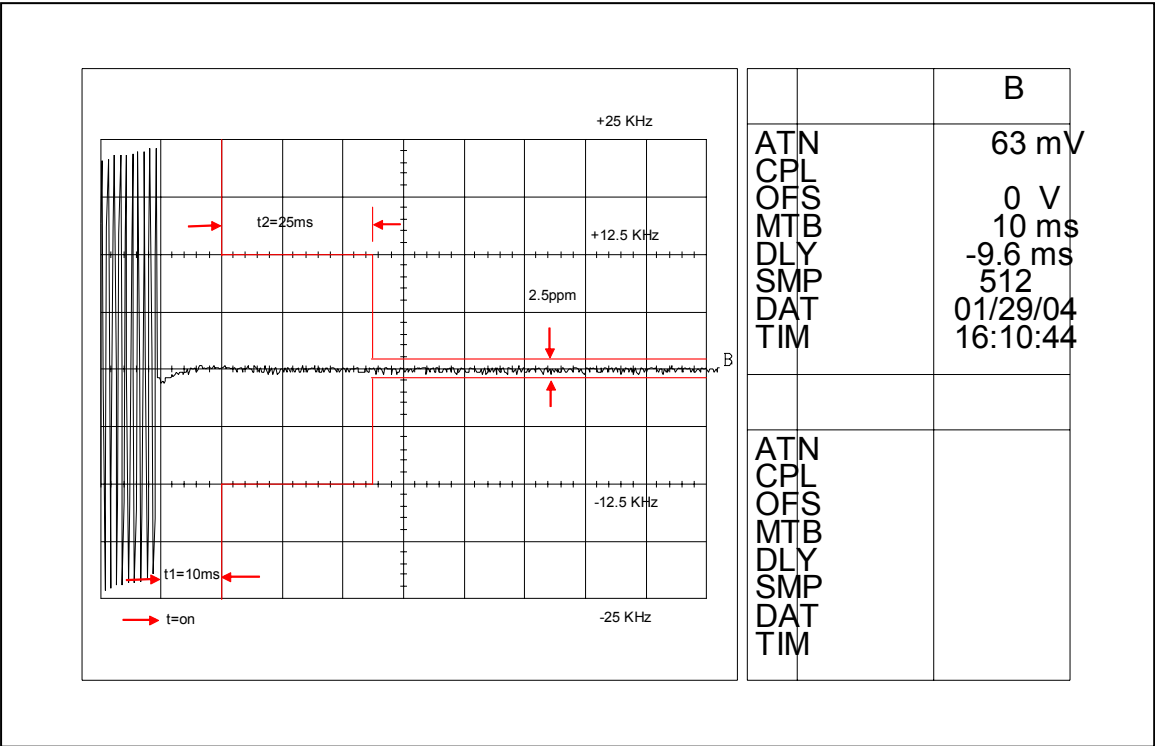
Figure 6I-7: 25 Watts, 25 KHz Key-Up Attack Time
