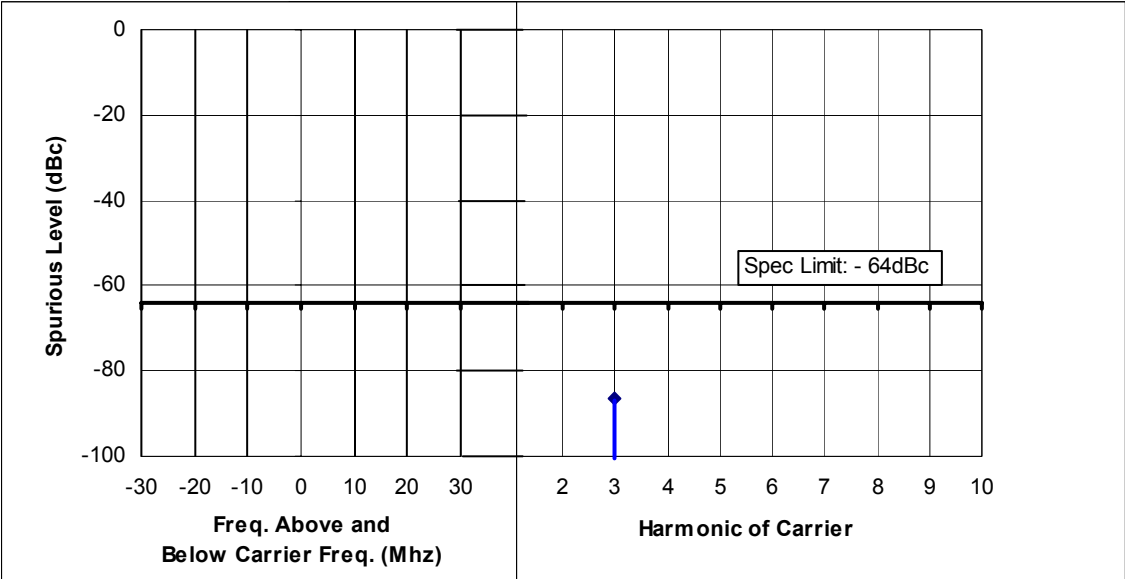
Figure 6F-9: 25 Watts, 439.975MHz, 12.5 kHz Channel Spacing
