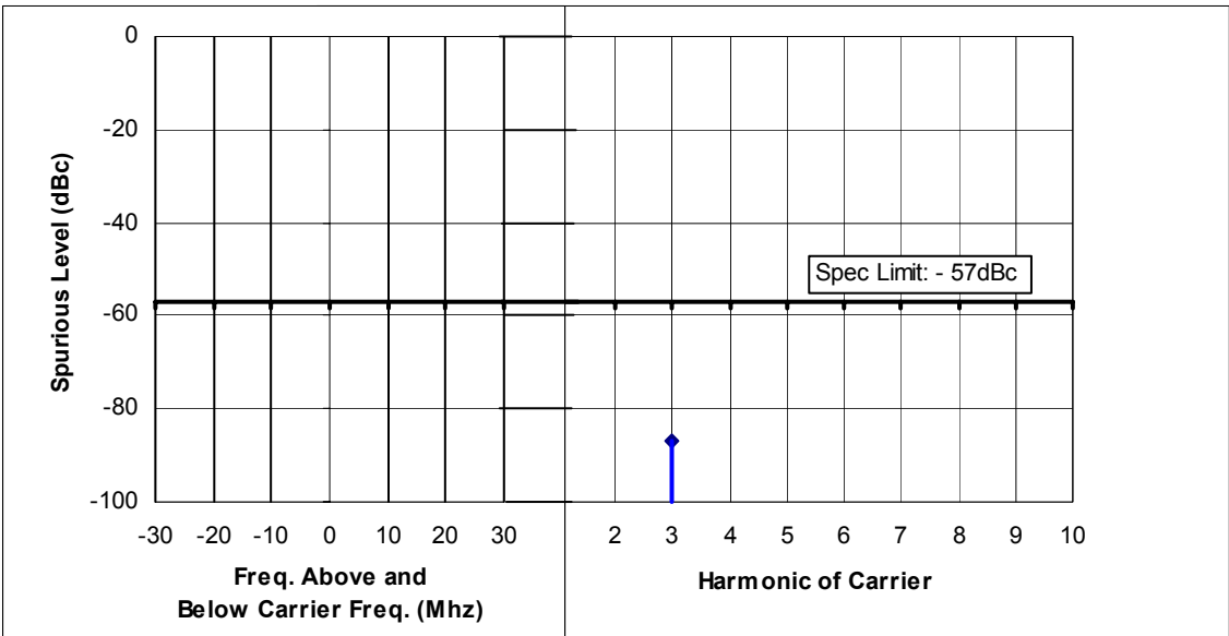
Figure 6F-12: 25 Watts, 439.975 MHz, 25 kHz Channel Spacing
