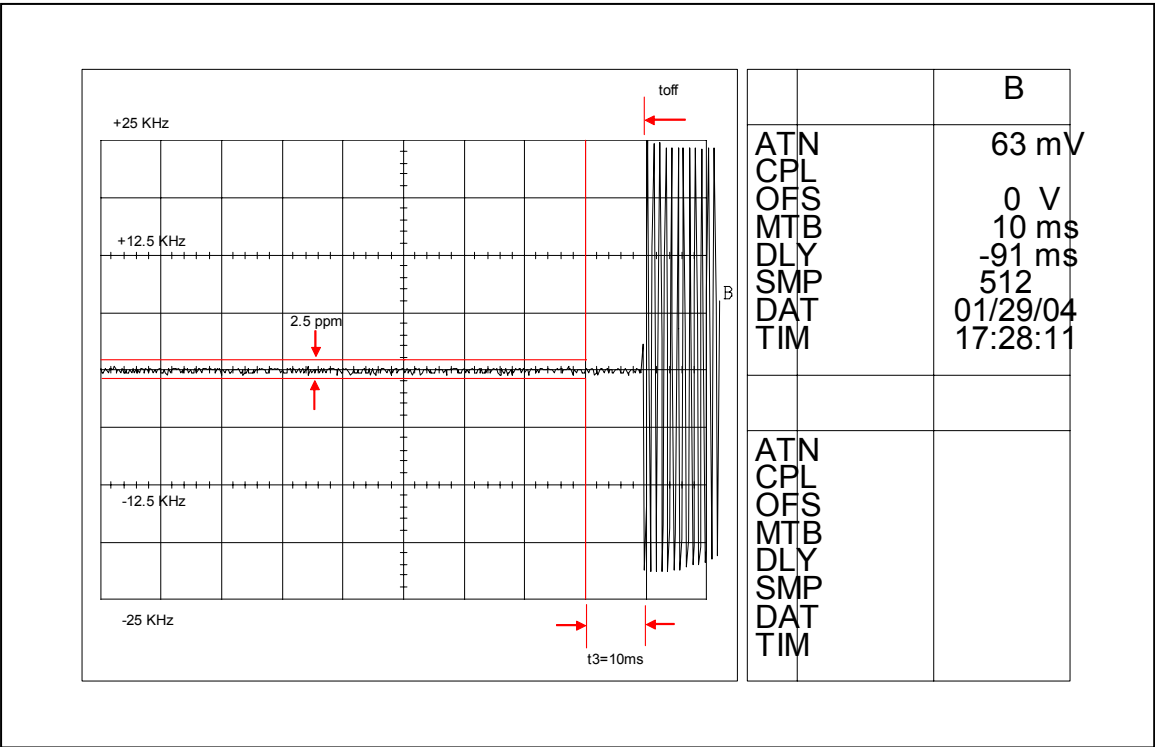
Figure 6I-8: 25 Watts, 25 KHz De-Key Decay Time
