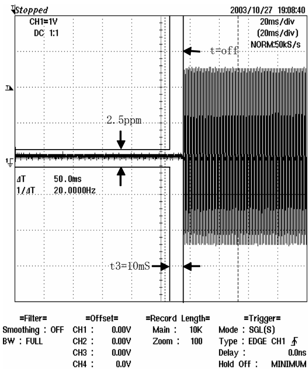
Figure 6I-4: 4 Watts, 25 KHz De-Key Decay Time
