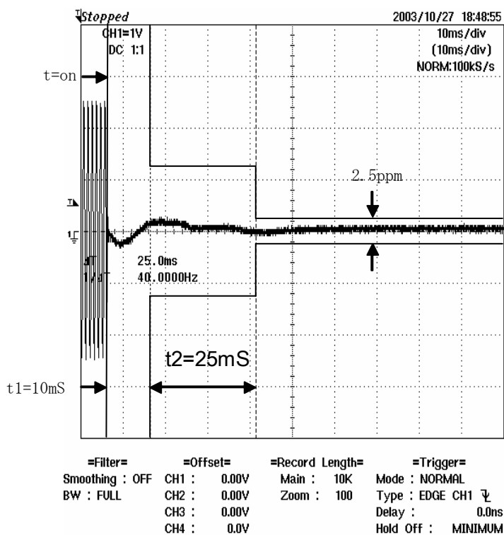
Figure 6I-3: 4 Watts, 25 KHz Key-Up Attack Time
