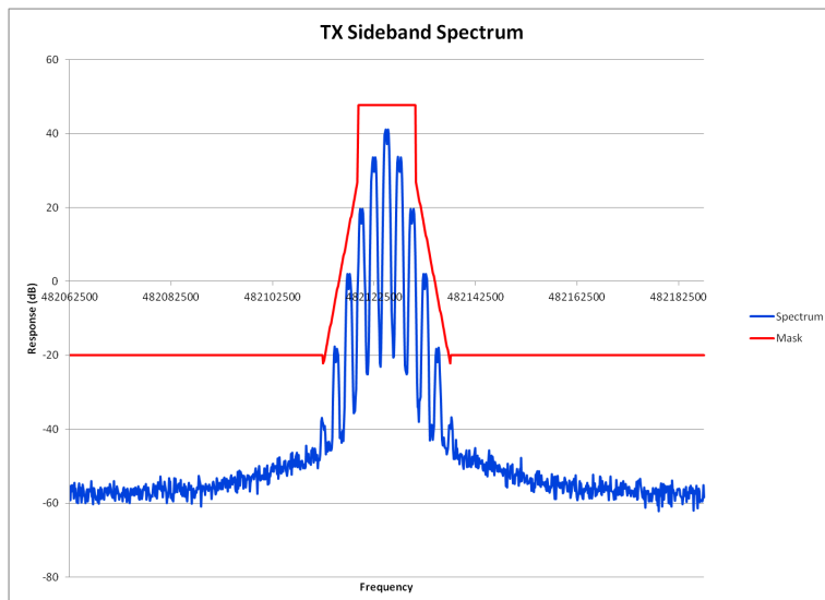
E1-5.35 Occupied Bandwidth, Analog, 12.5 kHz Channels, 482.125 MHz PL
