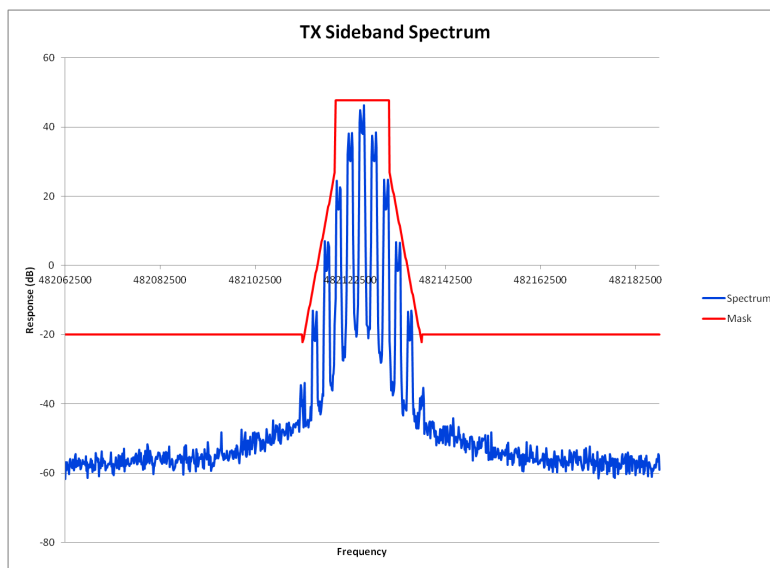
E1-5.36 Occupied Bandwidth, Analog, 12.5 kHz Channels, 482.125 MHz DPL
