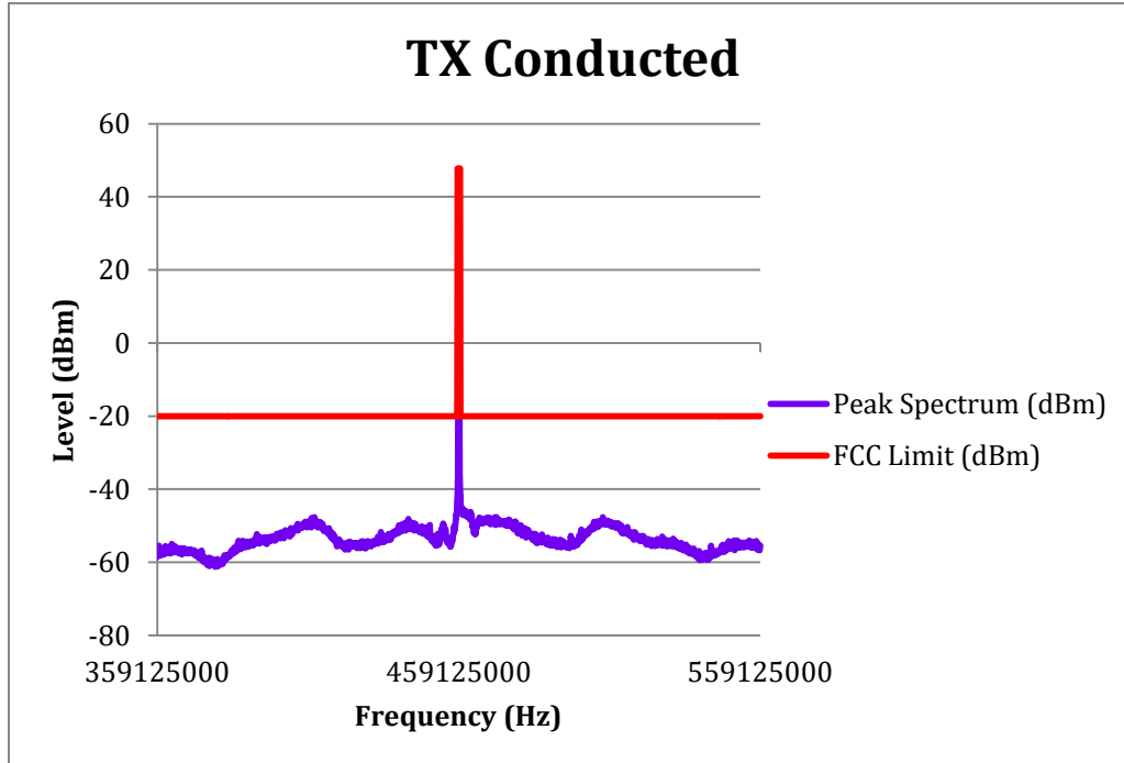
E1-6.4 Conducted Spurious Emission Spectrum, 200 MHz Span, Power 60 Watts, 459.125 MHz
