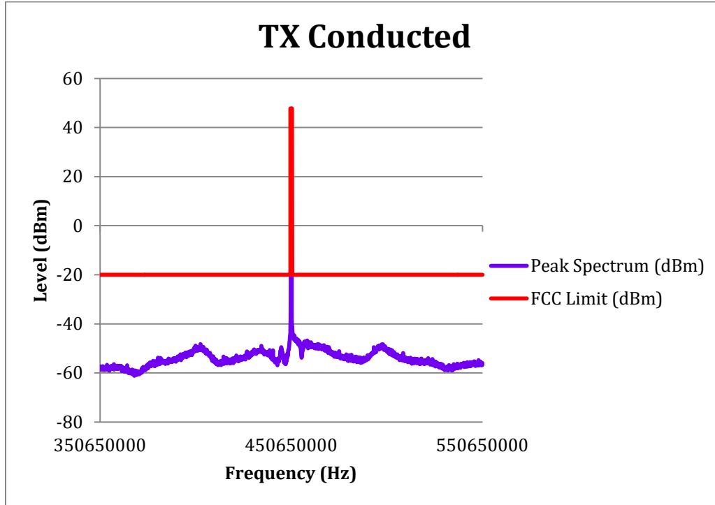
E1-6.3 Conducted Spurious Emission Spectrum, 200 MHz Span, Power 60 Watts, 450.65 MHz
