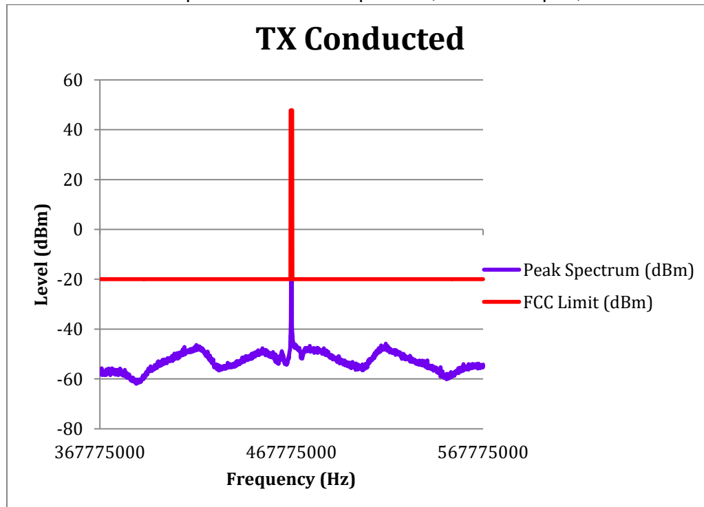
E1-6.5 Conducted Spurious Emission Spectrum, 200 MHz Span, Power 60 Watts, 467.775 MHz
