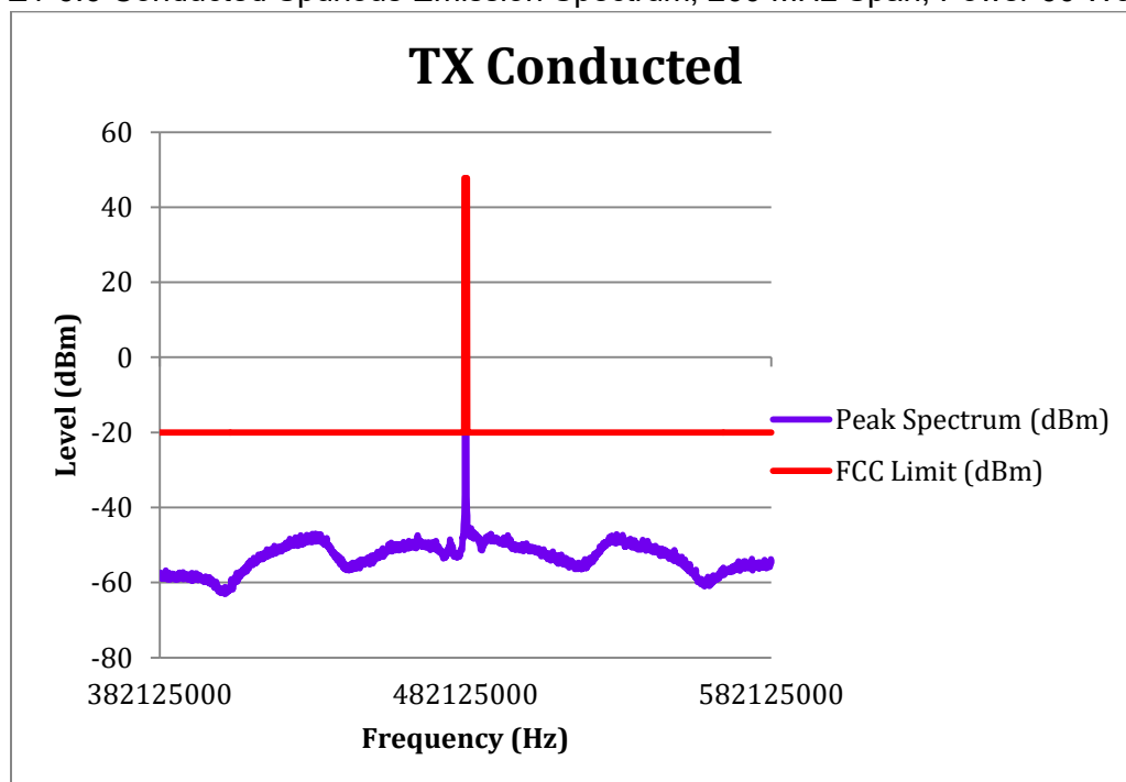
E1-6.6 Conducted Spurious Emission Spectrum, 200 MHz Span, Power 60 Watts, 482.125 MHz
