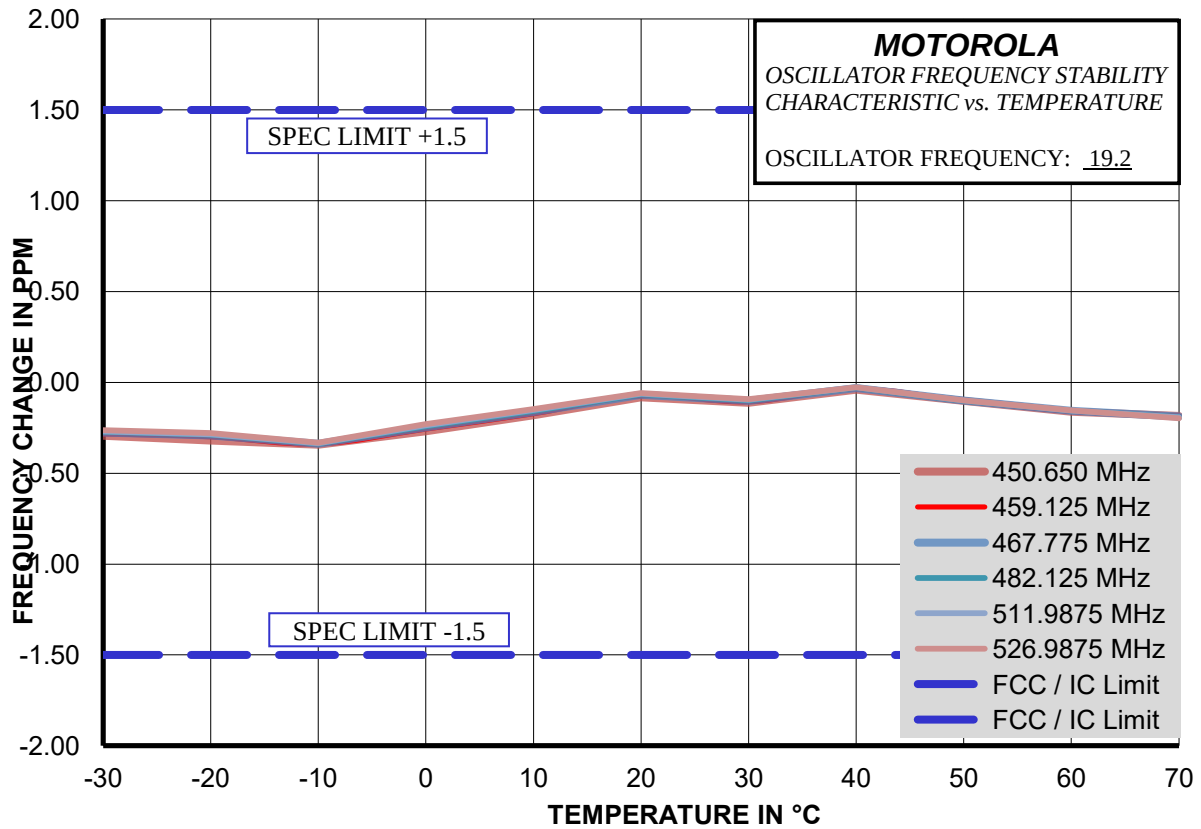
E1-8.1 Frequency Stability Vs Temperature
