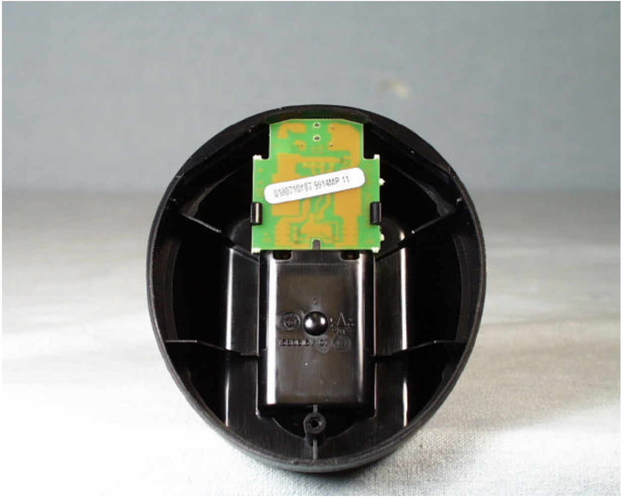
Bottom View of the Single Charger
