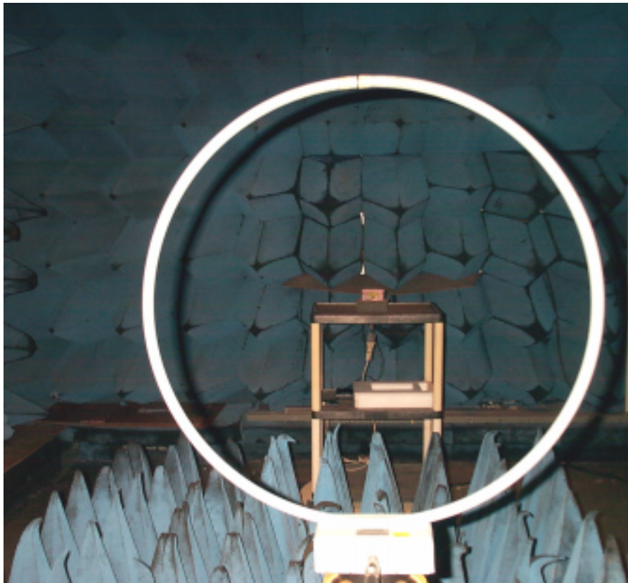
Figure E – 2 Radiated Emissions, Magnetic Loop, Test Setup - Chamber
