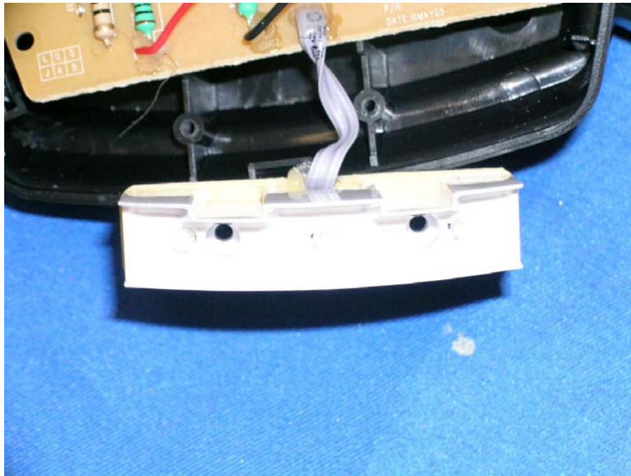
Base Charging Contacts front side
