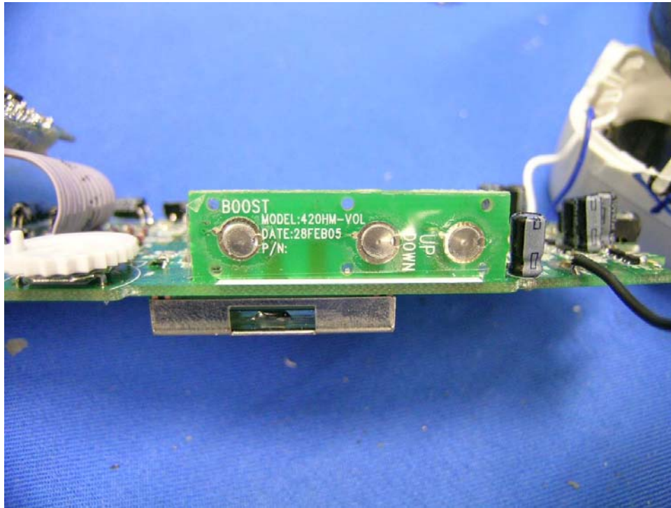
Handset UP/DOWN and BOOST Key front side
