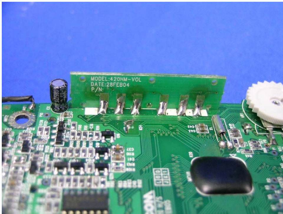
Handset UP/DOWN and BOOST Key rear side
