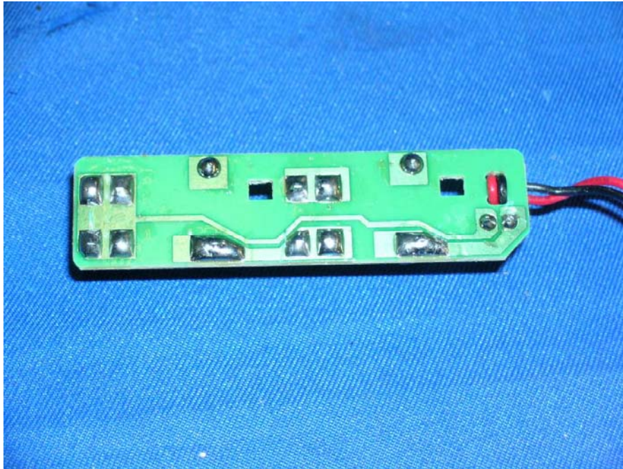
Base Unit Charger connect rear side
