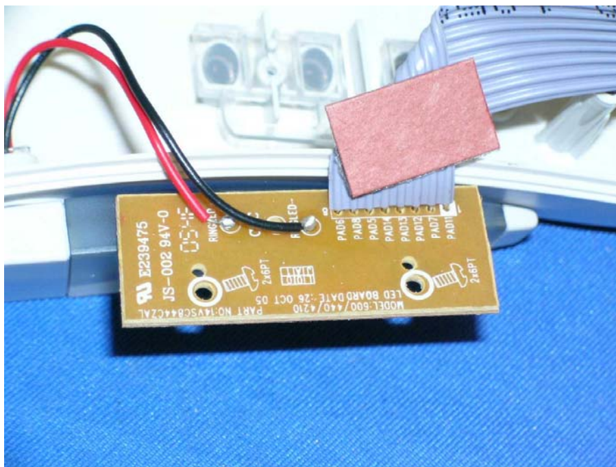
Base Unit LED front side
