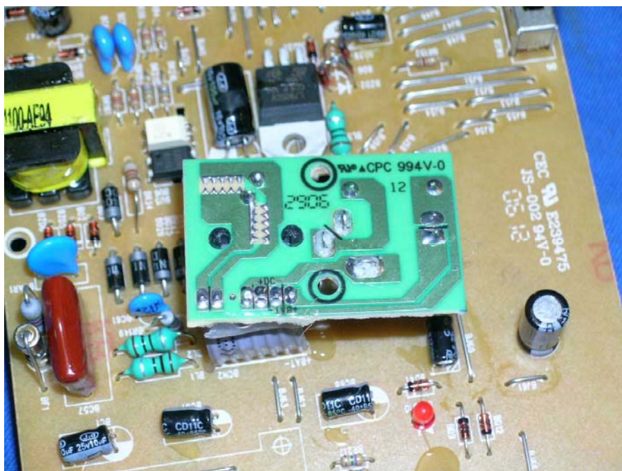
Base Unit Telephone Jack and AC Jack rear side
