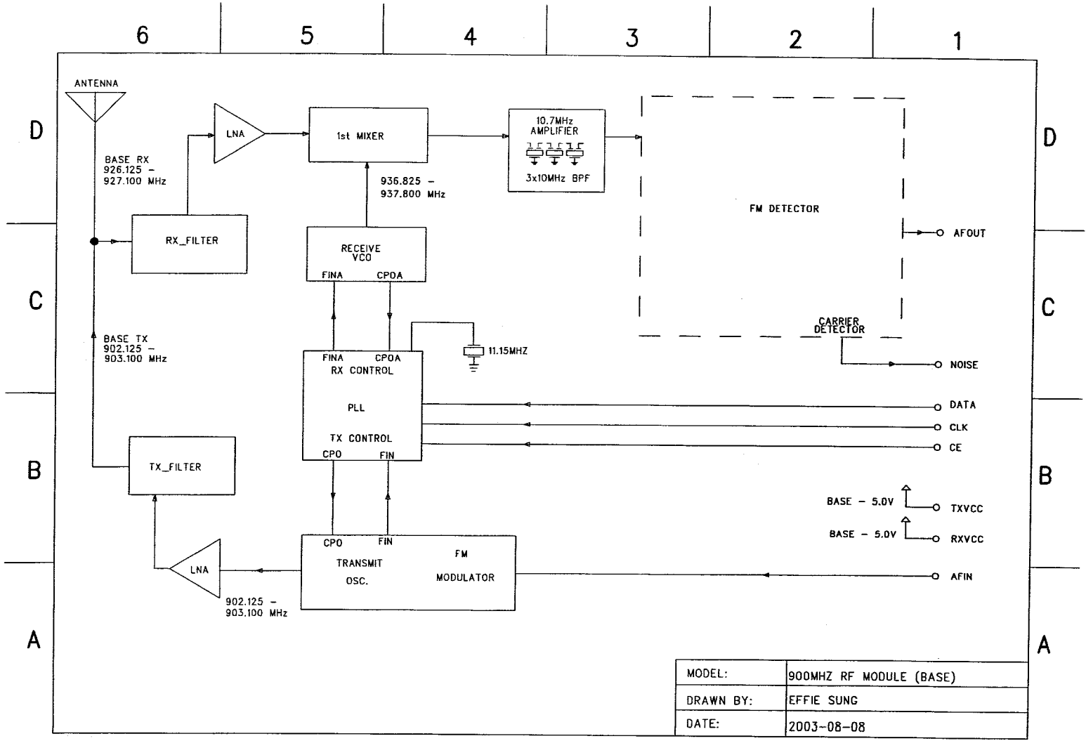
RF Module (Base) Block Diagram
