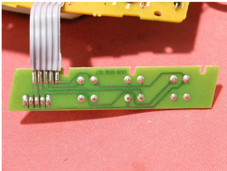
Base ring switch PCB rear side
