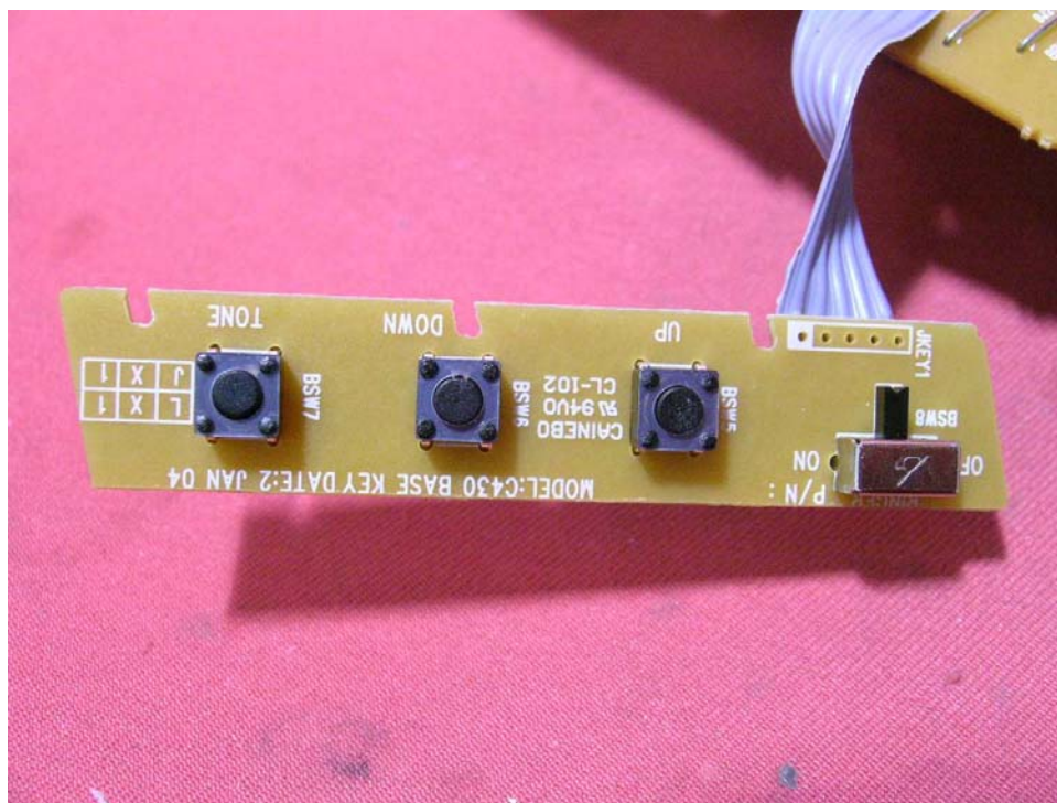
Base ring switch PCB front side
