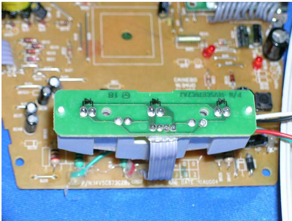
Base Charging Contacts rear side
