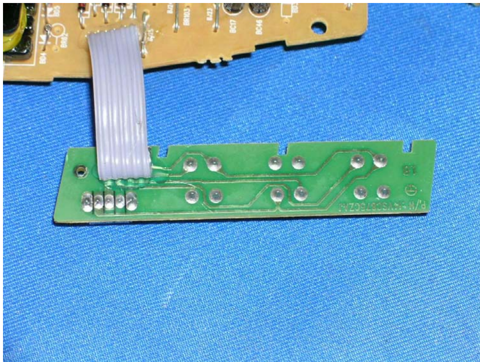
Base Ringer Off/On, Volume Up/Down and Ring Style Key rear side
