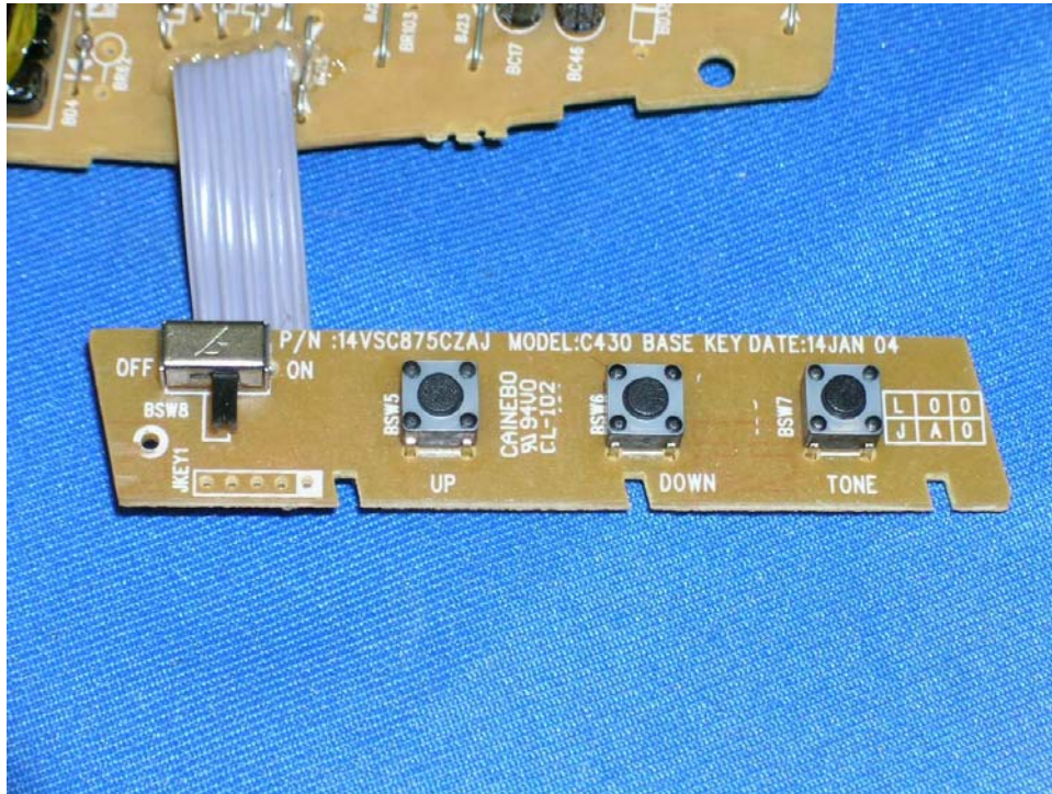
Base Ringer Off/On, Volume Up/Down and Ring Style Key front side
