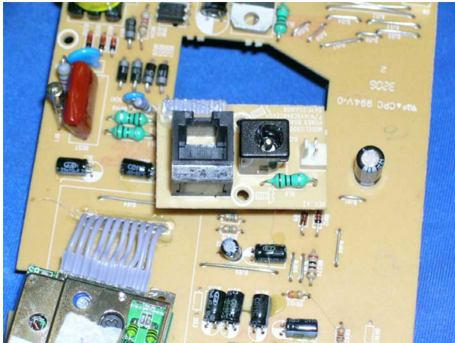
Base Unit Telephone Jack and AC Jack front side
