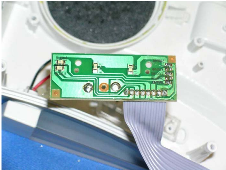
Base Unit LED PCB rear side
