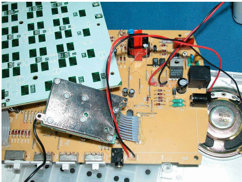
Base Main PCB comp side (View 3)
