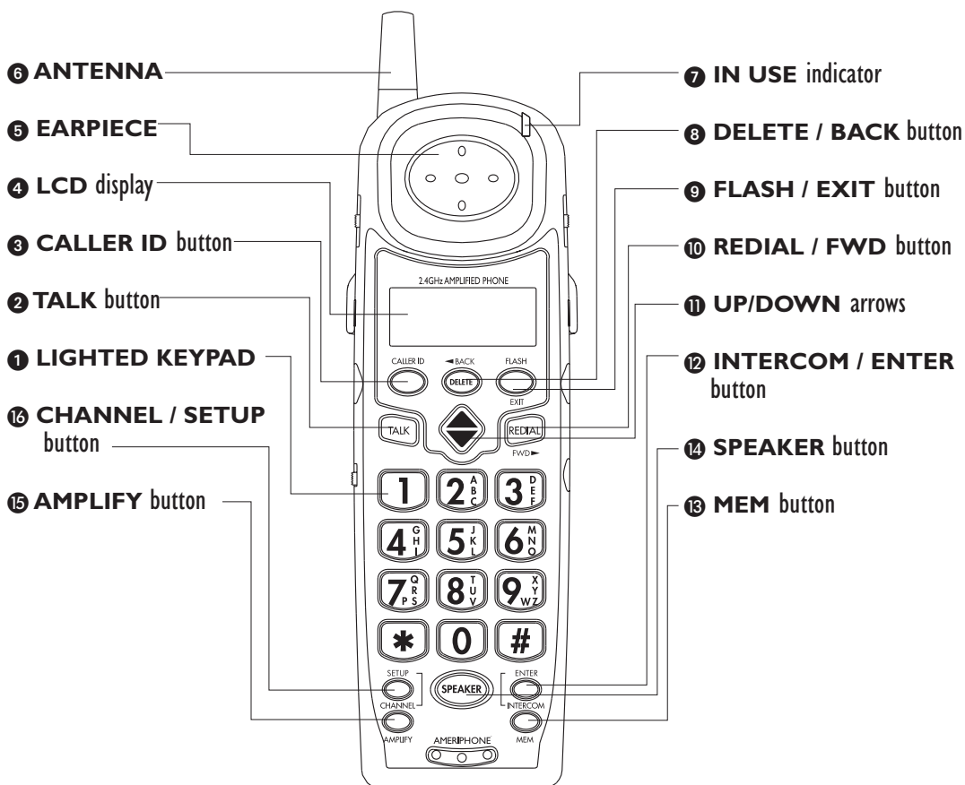
Handset Face
