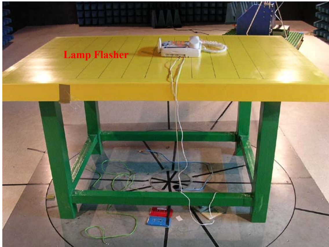
Photo 2: Tx Radiated Emission Set-up Photo
