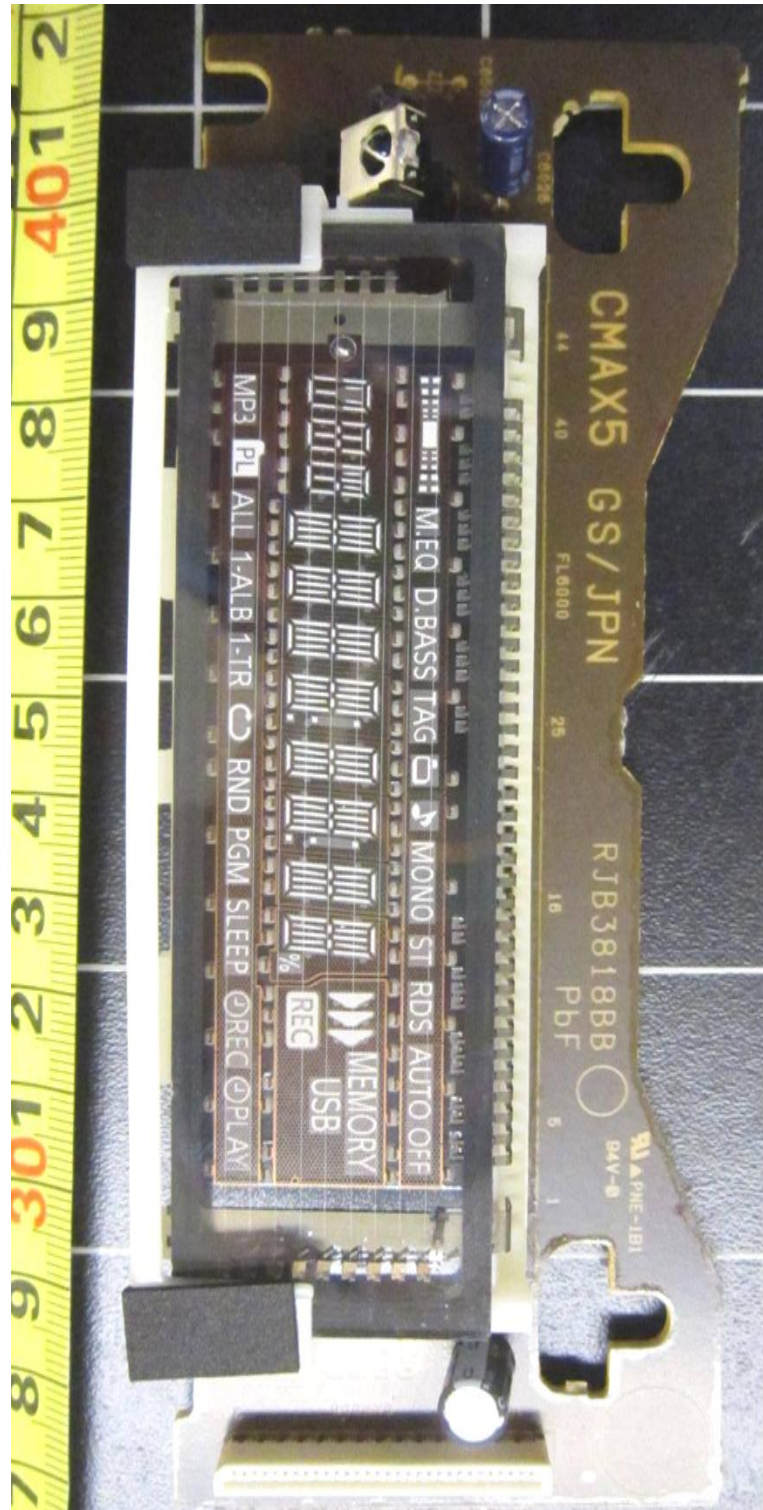
LCD Display Board PCB Component Side
