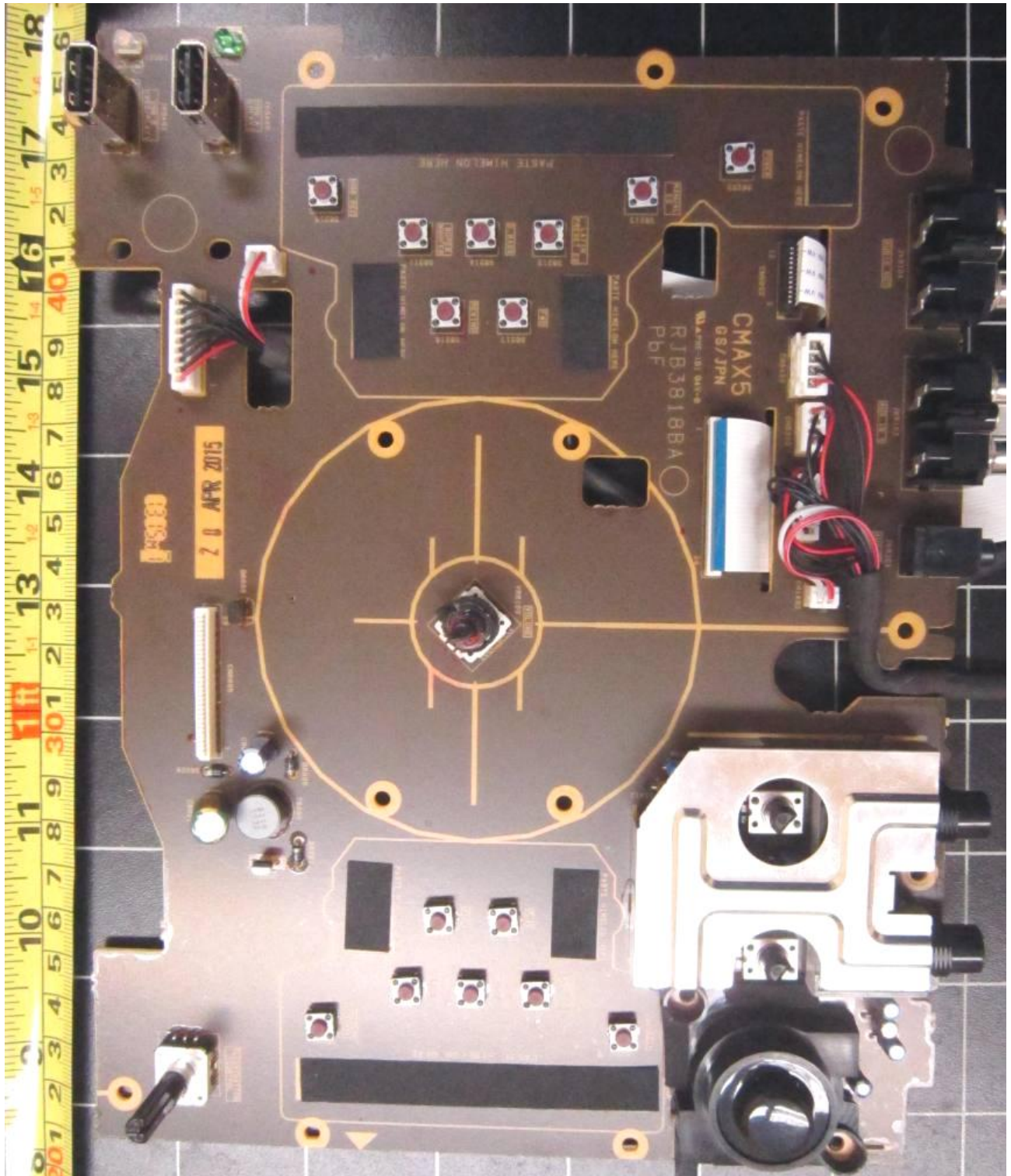
Main-Board PCB Component Side
