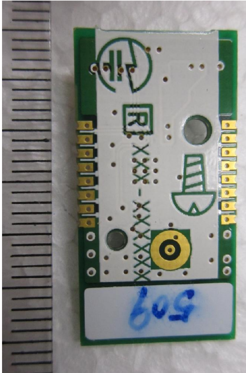
RF Module Circuit Trace Side
