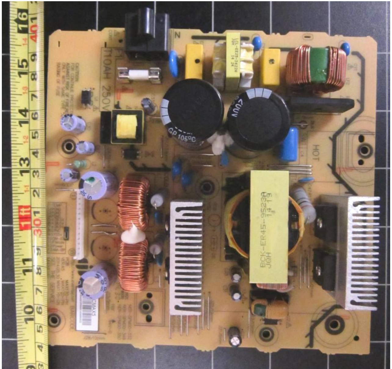
Power Supply Sub-Board PCB Component Side
