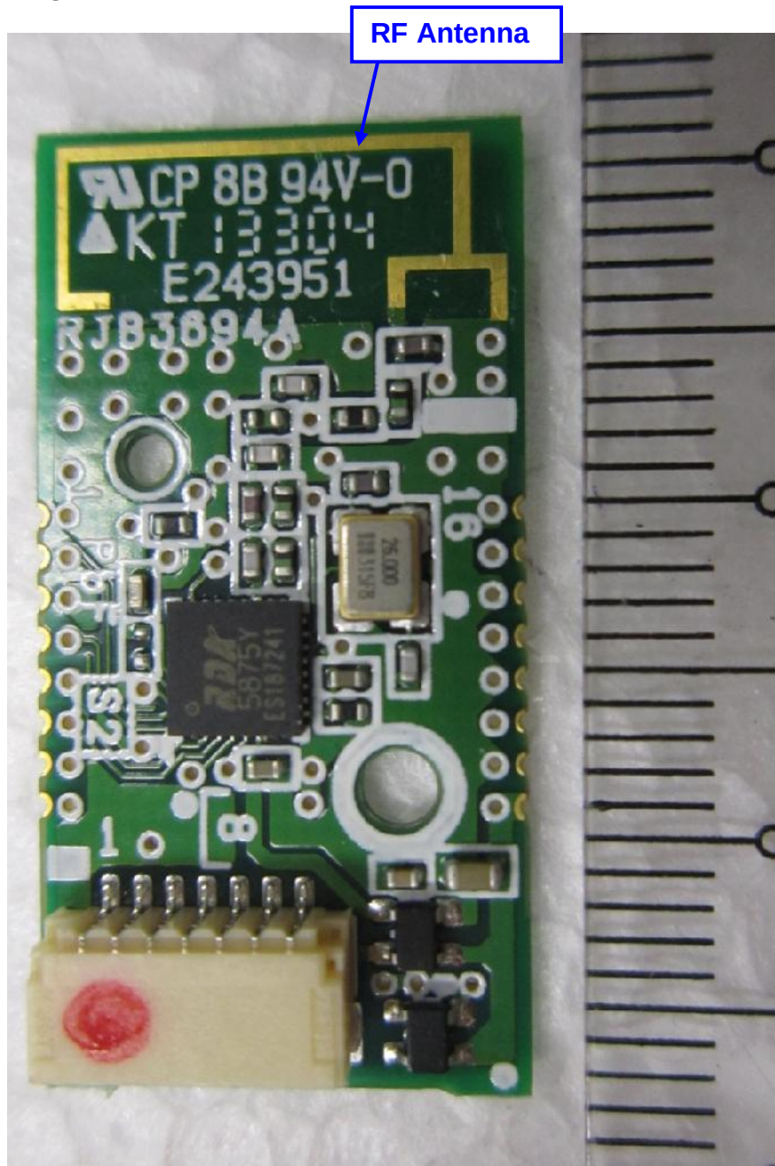
RF Module Circuit Component Side
