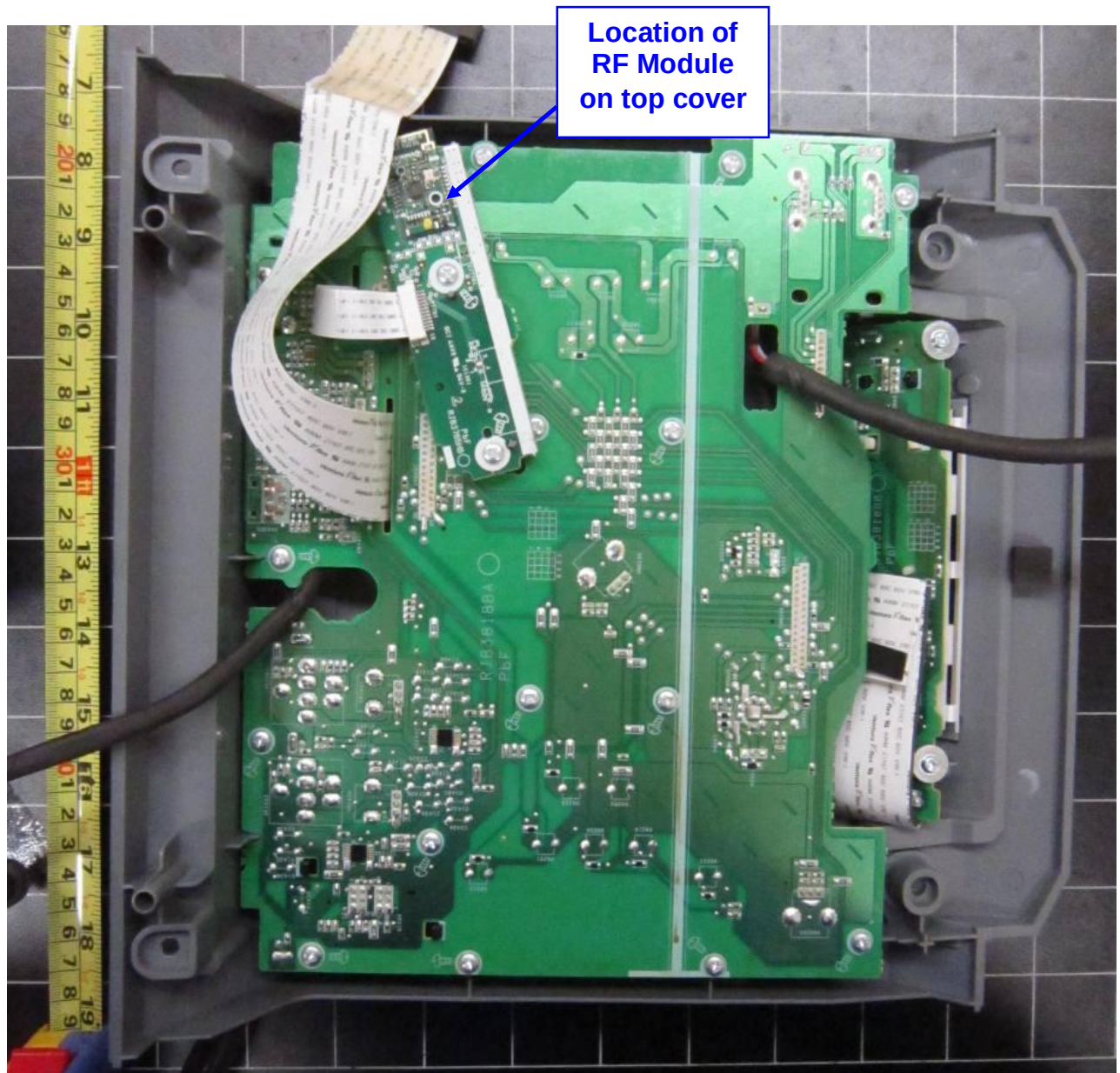
Internal View 2
