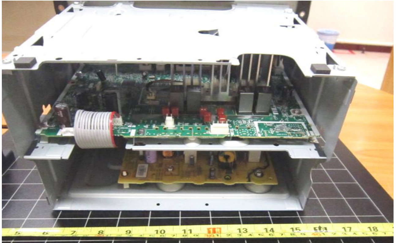
Internal View 3
