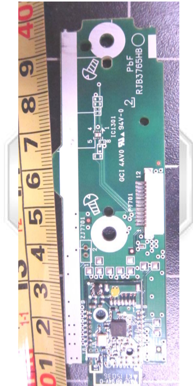
Sub-Board PCB Component Side
