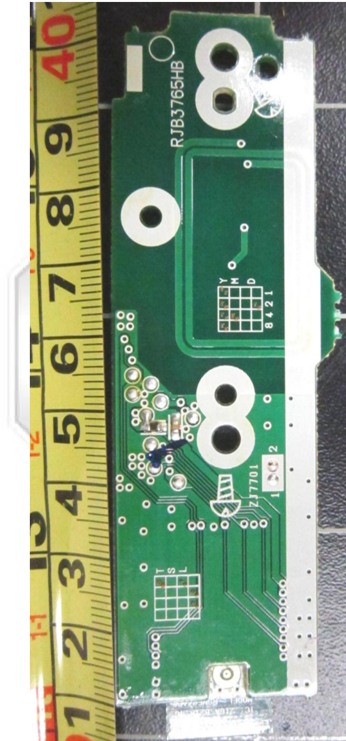
Main-Board PCB Trace Side
