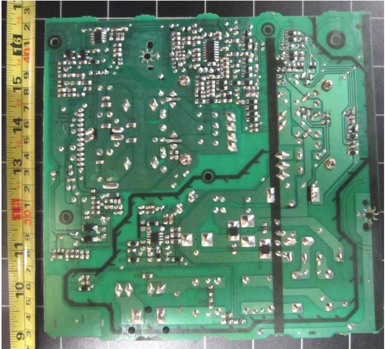
Power Supply Sub-Board PCB Trace Side
