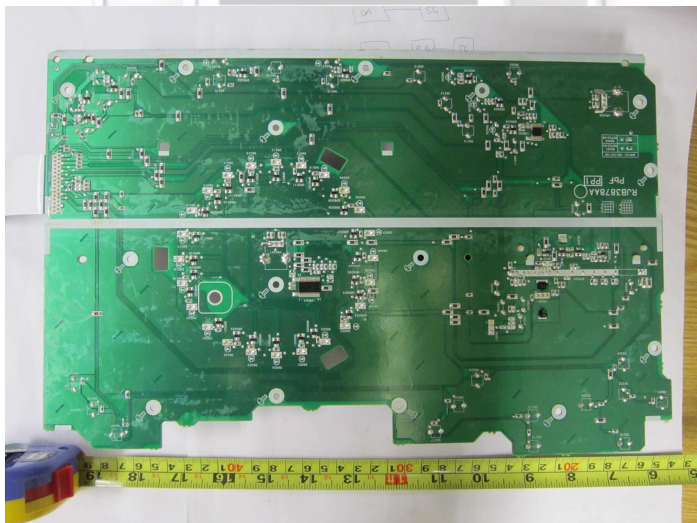
LCD Display Board PCB Trace Side
