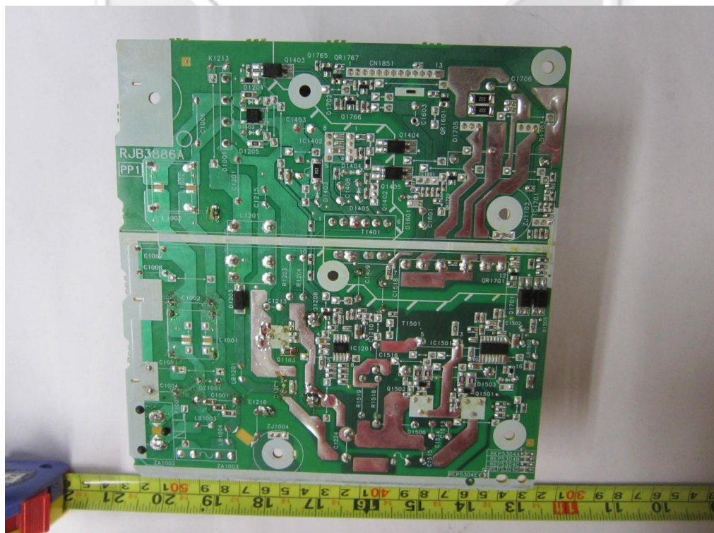
Power Supply Board PCB Trace Side
