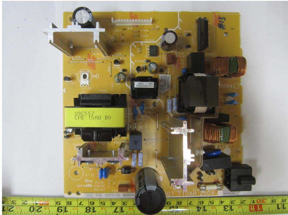
Power Supply Board PCB Component Side
