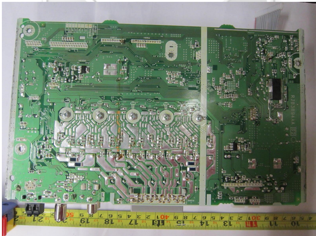
Main-Board PCB Trace Side
