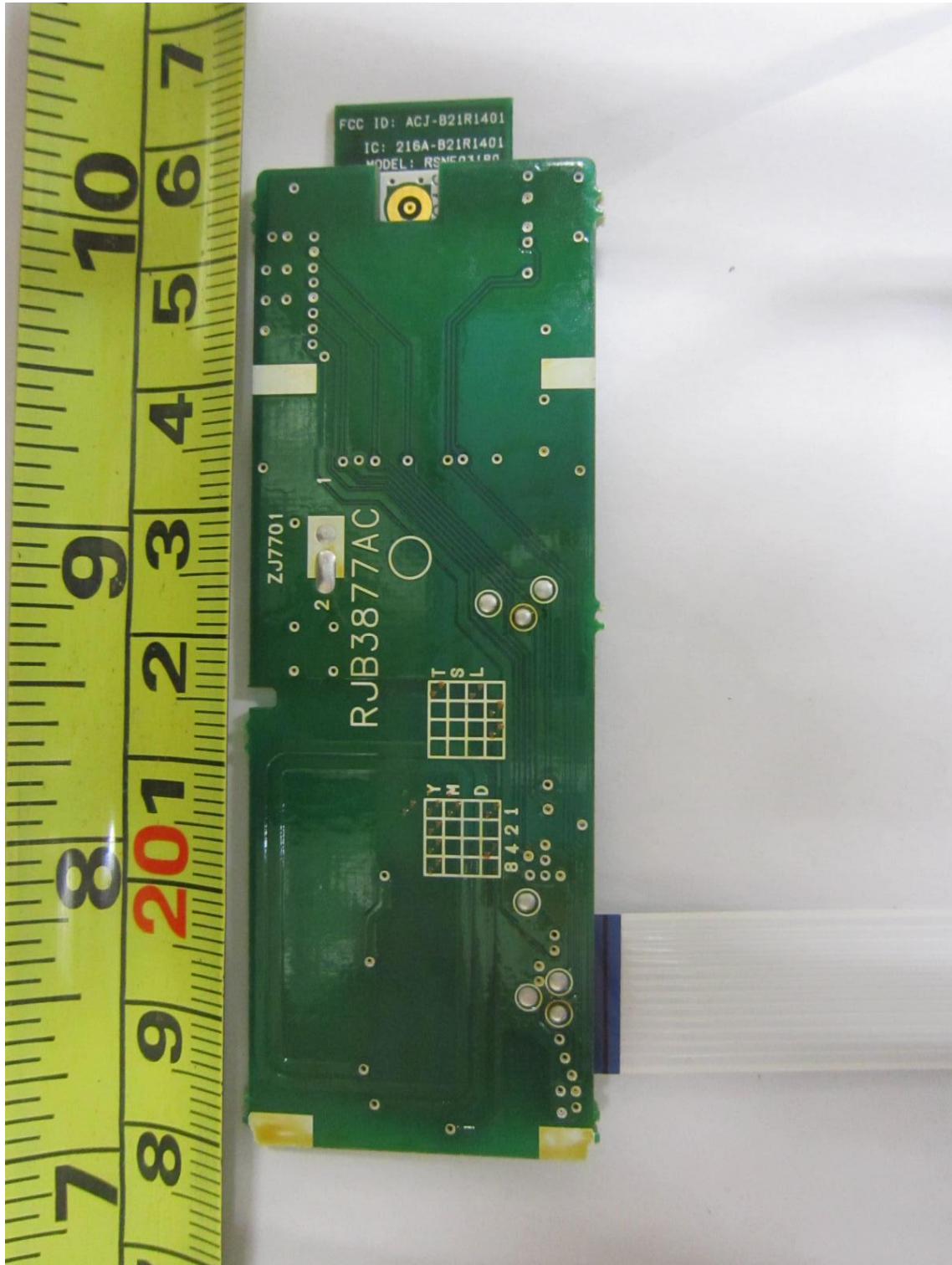
RF Module Circuit Trace Side
