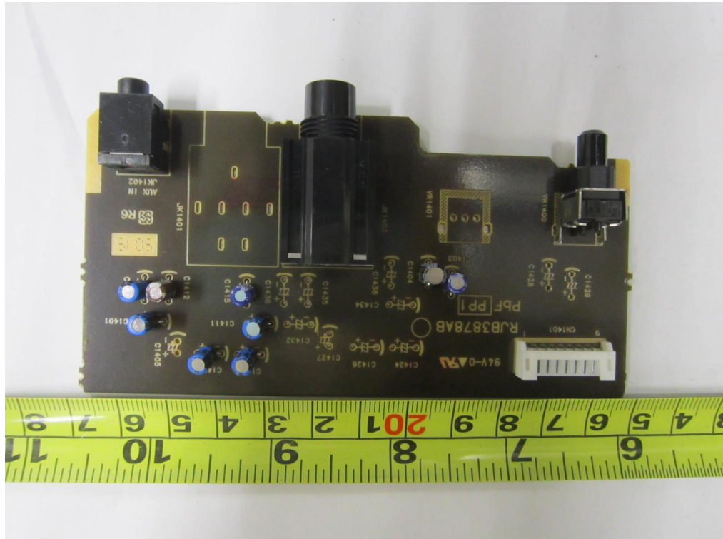
Sub-Board 1 PCB Component Side
