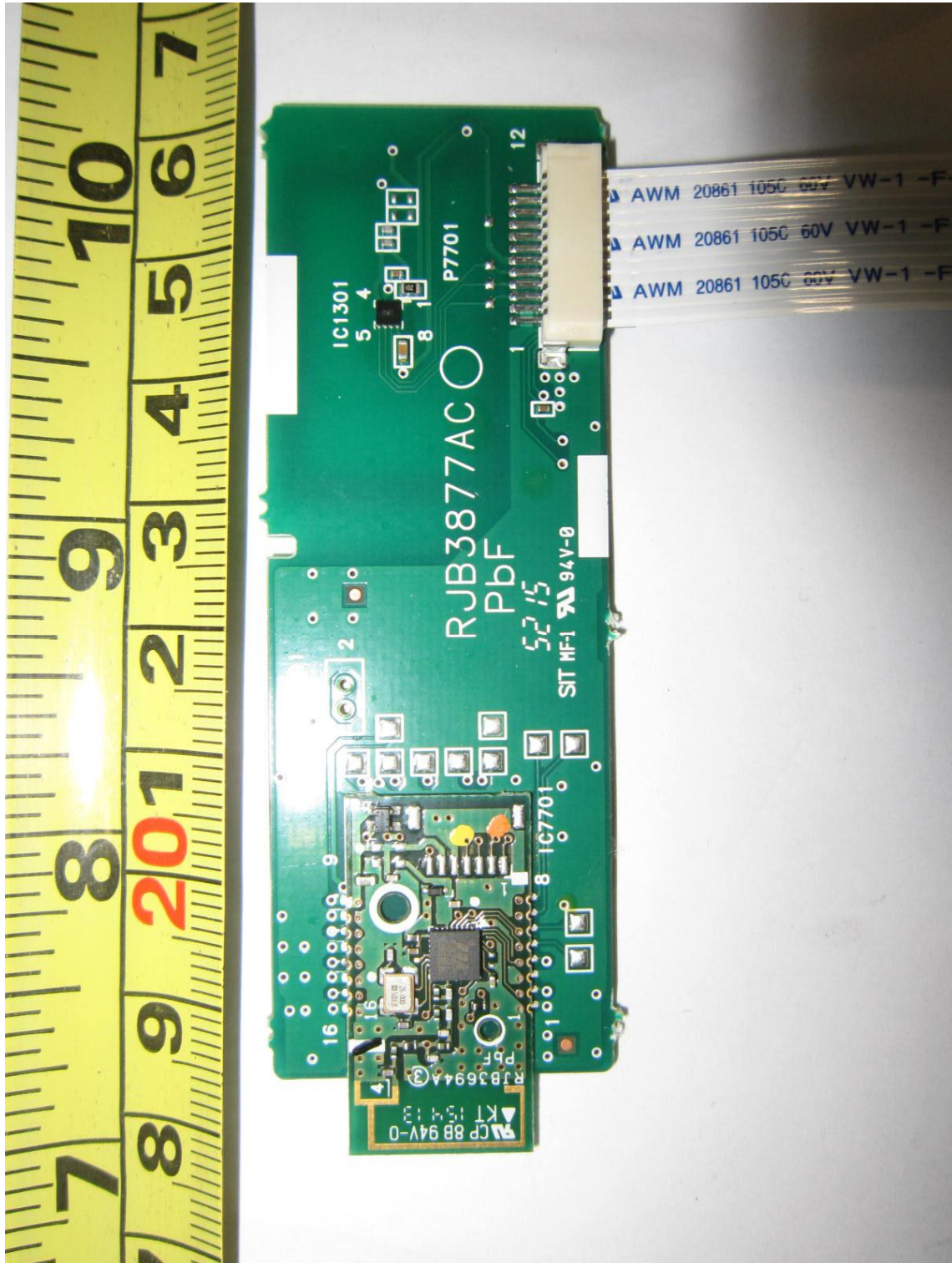
RF Module Circuit Component Side
