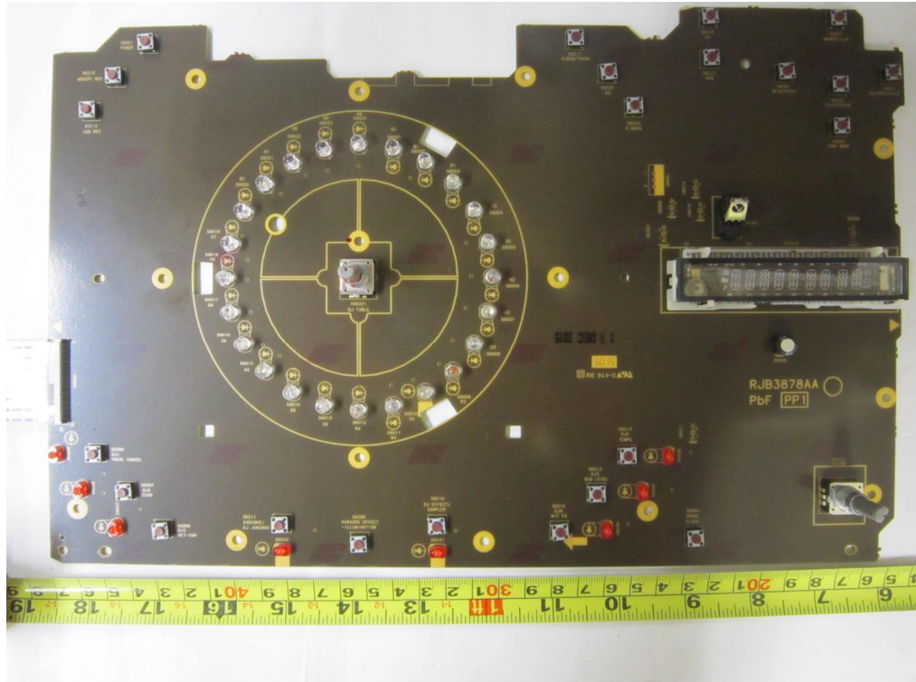
LCD Display Board PCB Component Side
