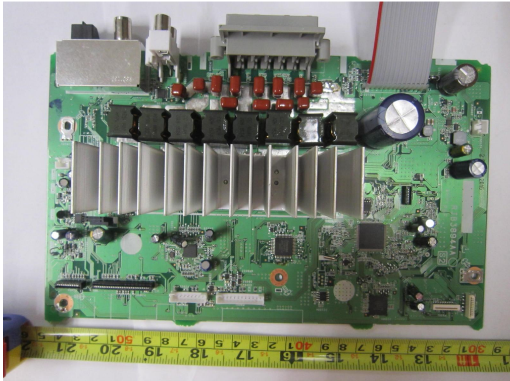
Main-Board PCB Component Side
