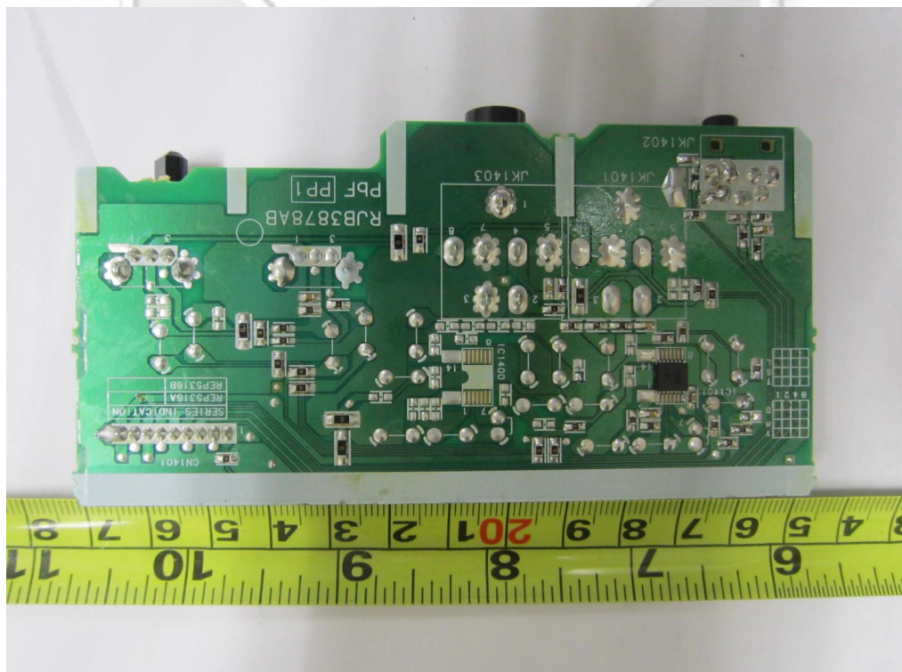
Sub-Board 1 PCB Trace Side
