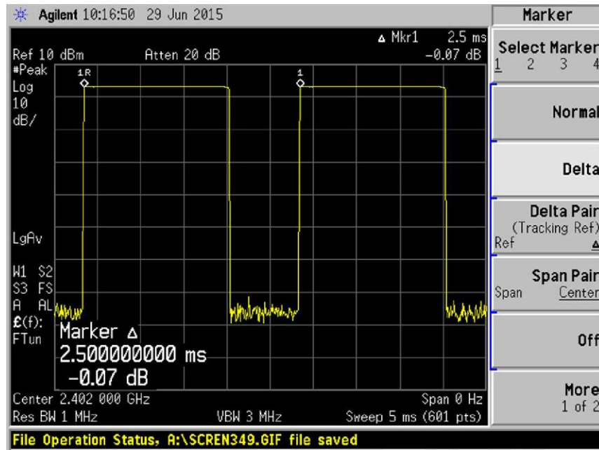
Plot 21 – Channel 0 (lower ch)
