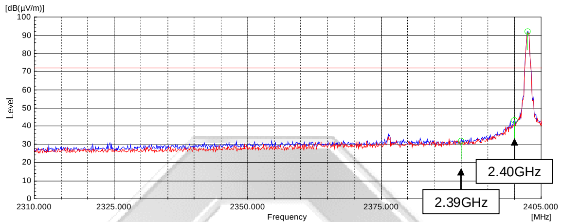
Plot 51 – Lower Band Edge at 2.4000GHz
