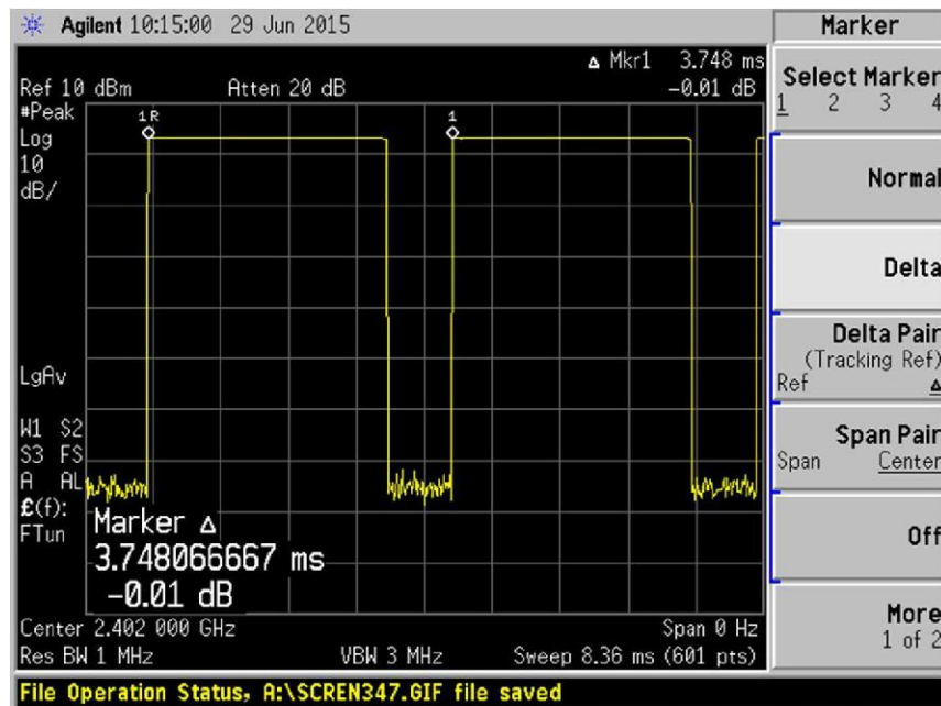
Plot 24 – Channel 0 (lower ch)
