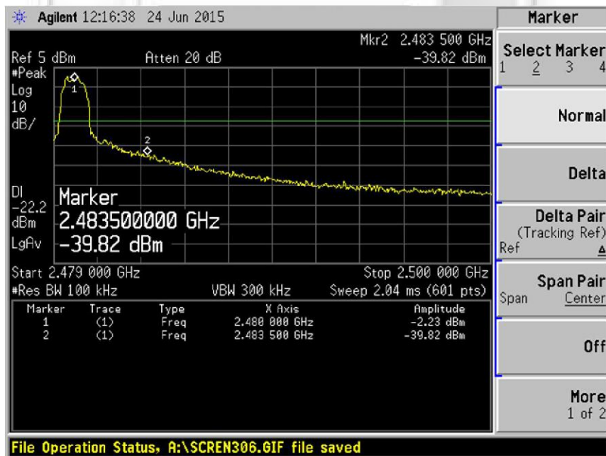
Plot 48 – Upper Band Edge at 2.4835GHz
