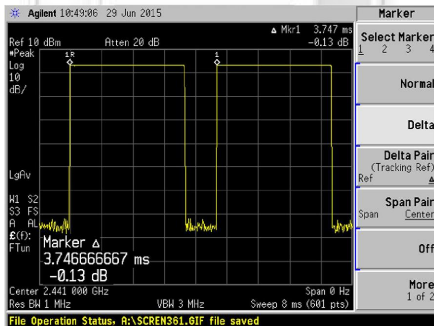
Plot 25 – Channel 39 (mid ch)
