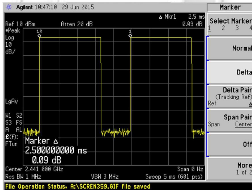
Plot 22 – Channel 39 (mid ch)
