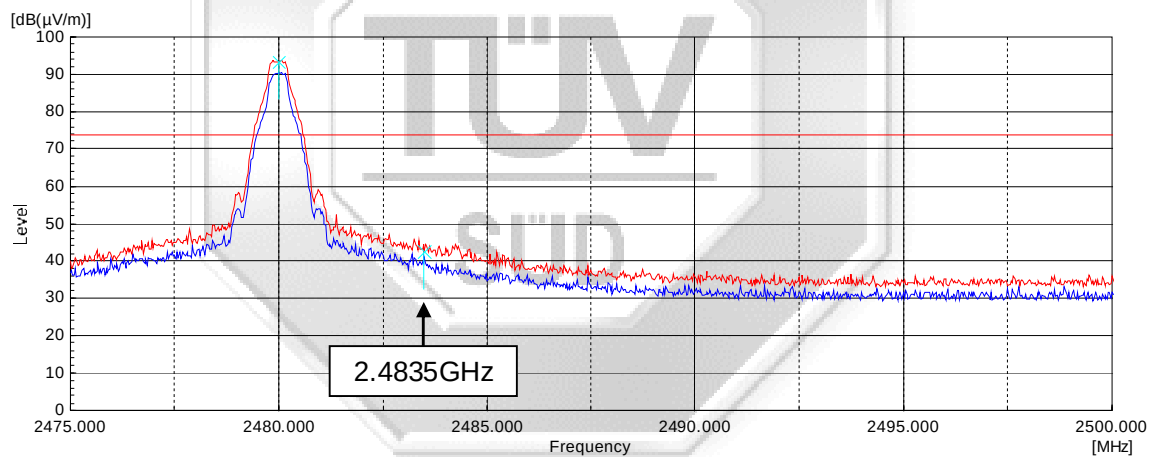
Plot 52 – Upper Band Edge at 2.4835GHz
