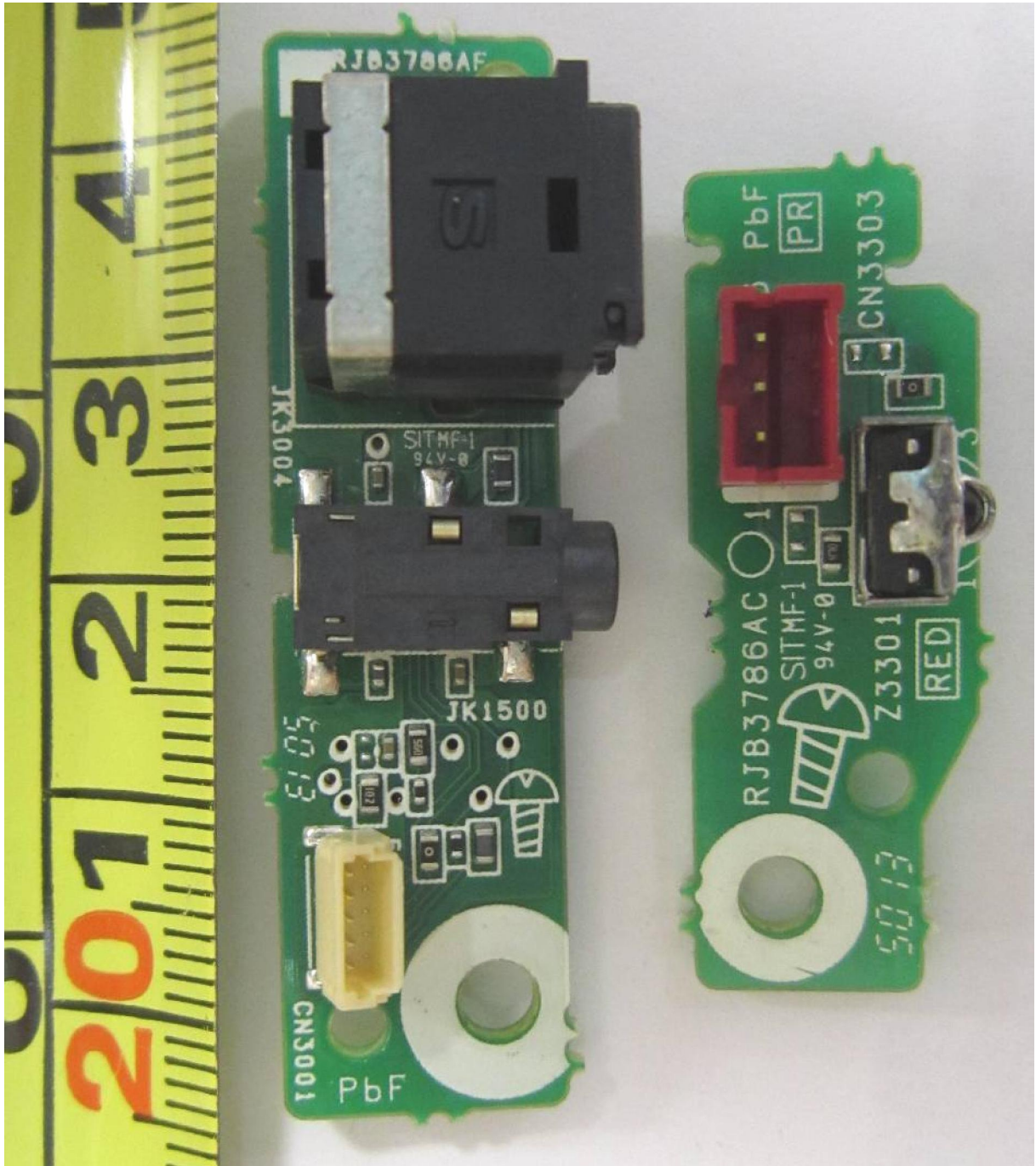
Sub-Board 4 PCB Component Side
