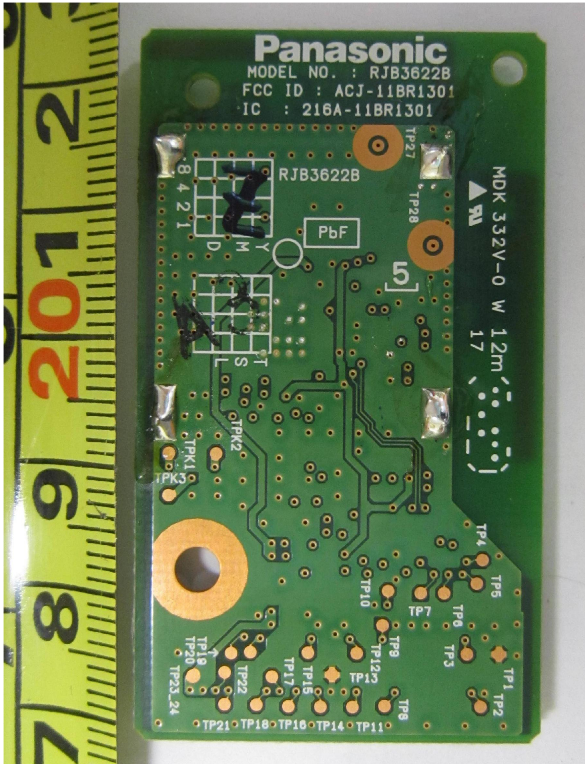
RF Receiver Module PCB Trace Side
