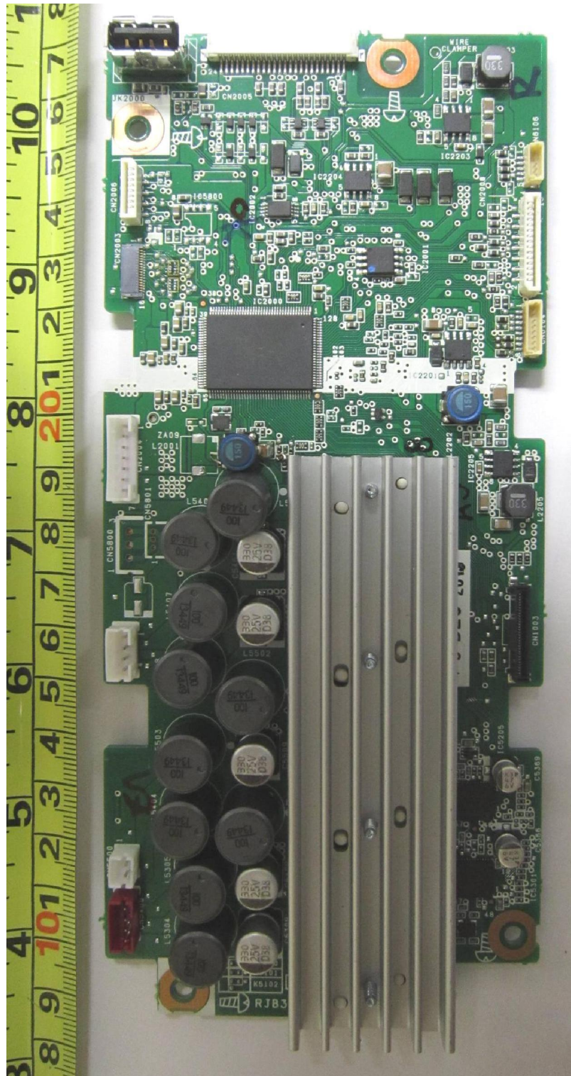
Main-Board PCB Component Side
