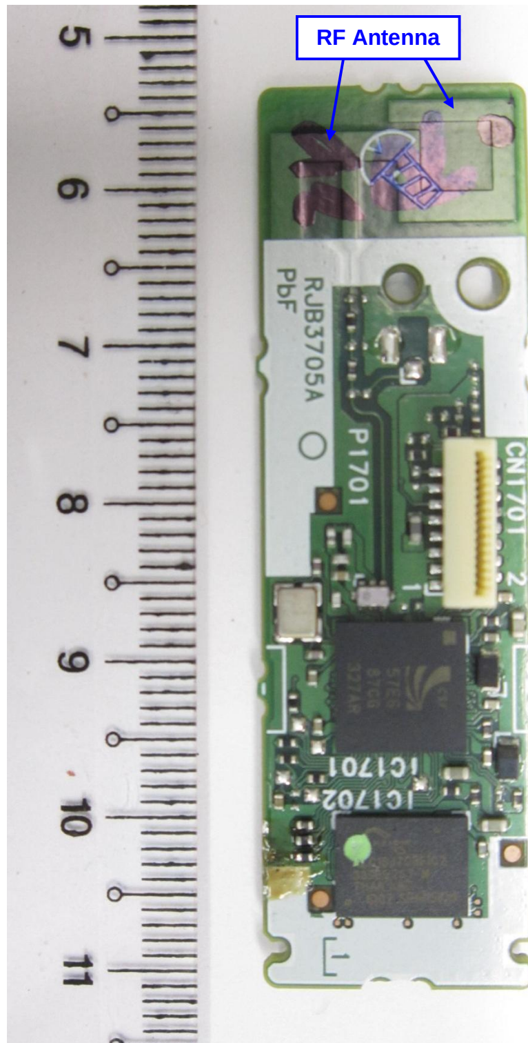
Bluetooth Module PCB Component Side
