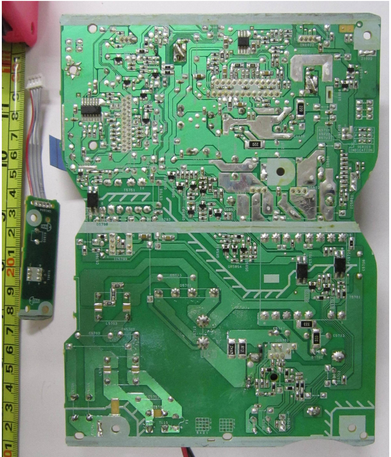
Main-Board PCB Trace Side
