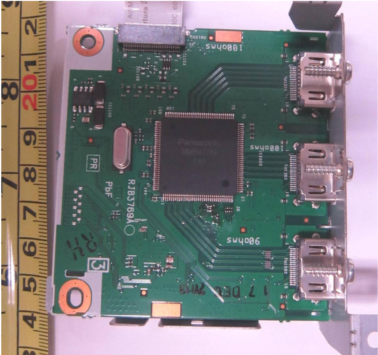
Sub-Board 1 PCB Component Side
