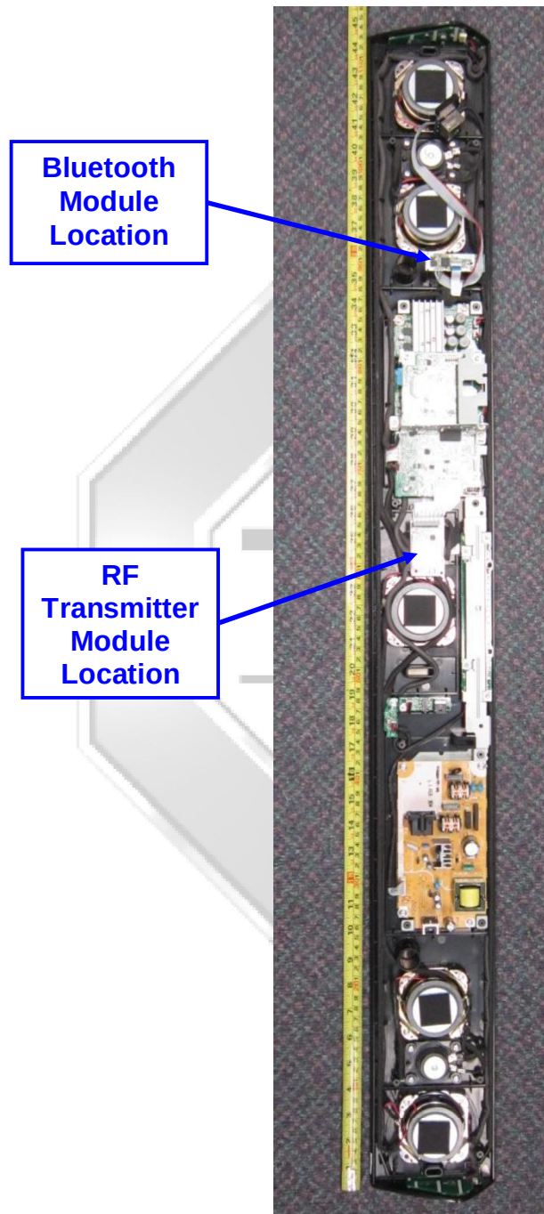
EUT Internal View
