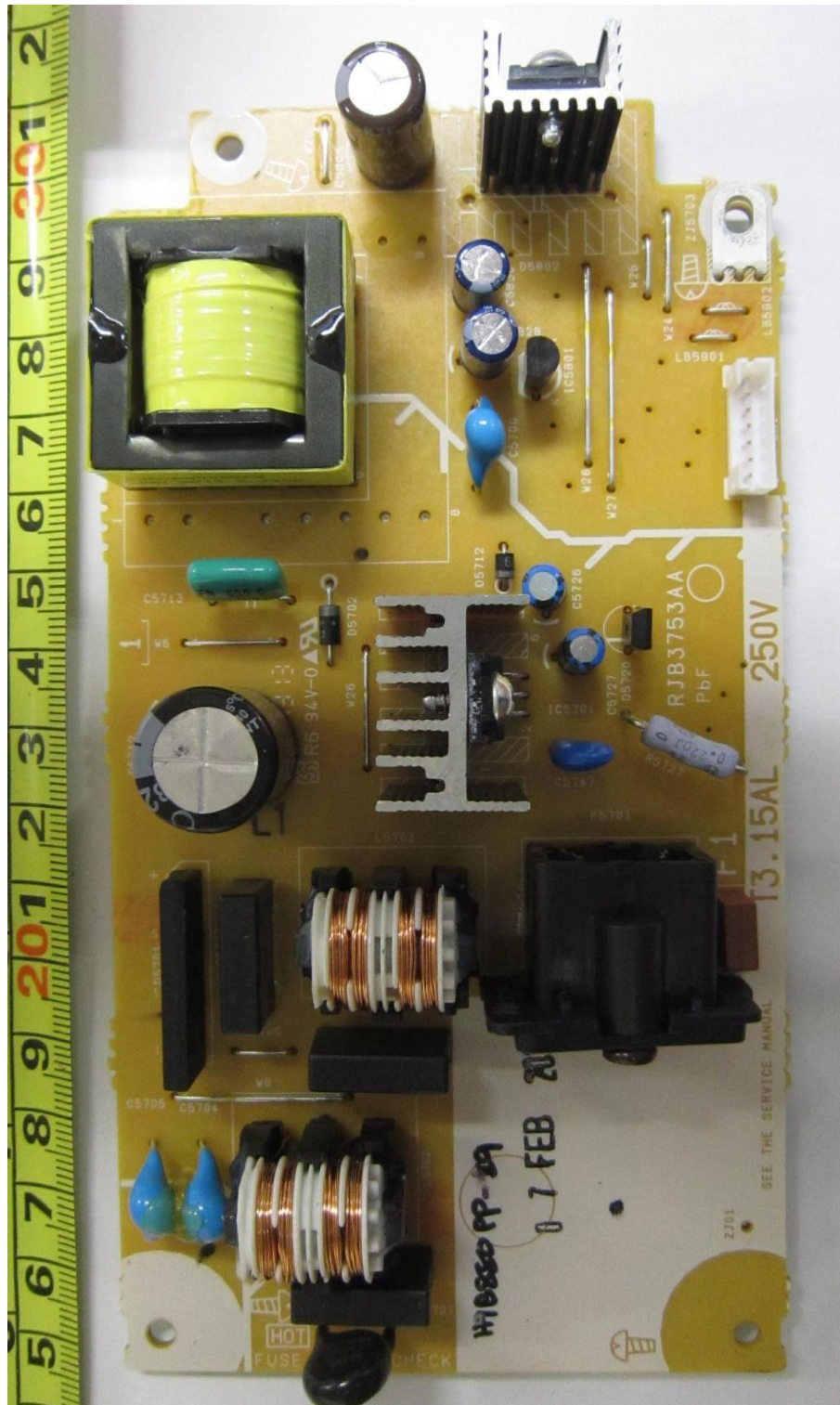
SMPS Board PCB Component Side
