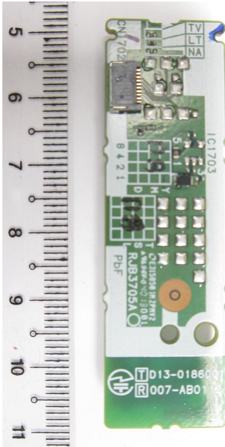
Bluetooth Module PCB Trace Side
