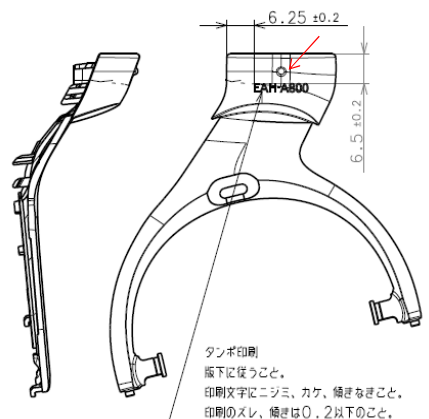
HANGER INNER L
