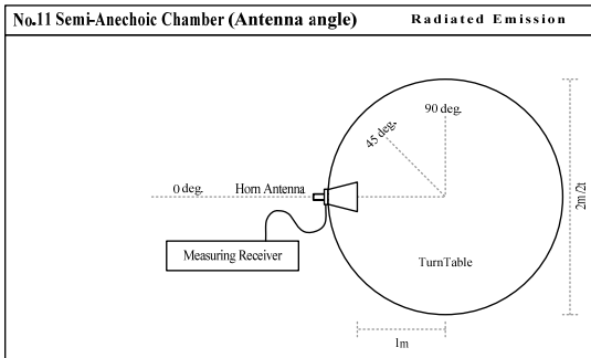
Above13GHz
