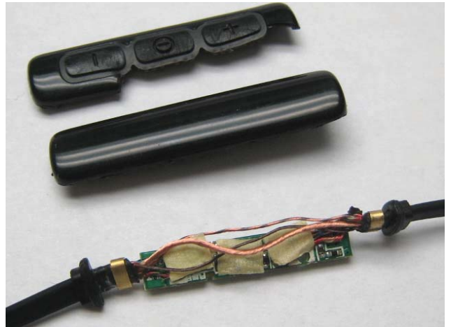
Controller
