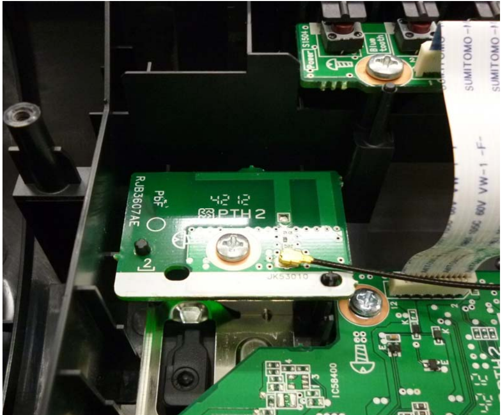
Detail View of AirPlay Antenna
