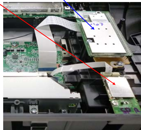
Bottom Side View
