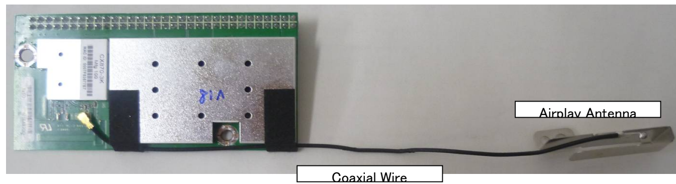
Antenna Connection
