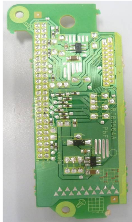
Bottom View
