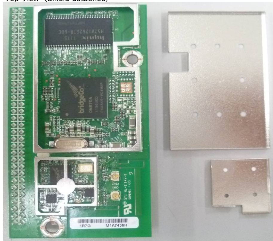
Top View (Shield detached)
