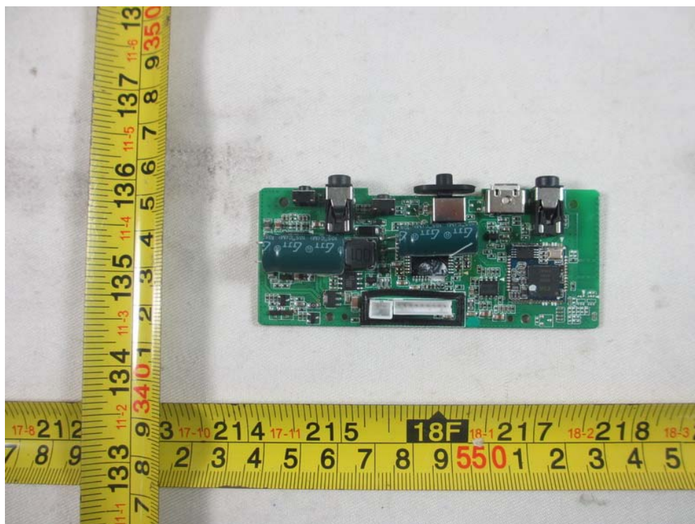
Accessory Board
