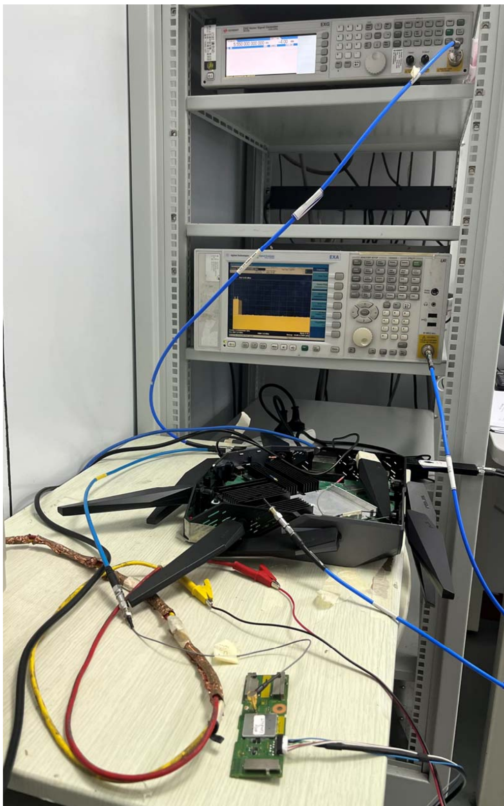
Picture 1 DFS Test Setup
