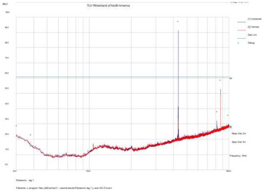
Figure 19: 30MHz-1000MHz, 433.272 MHz
