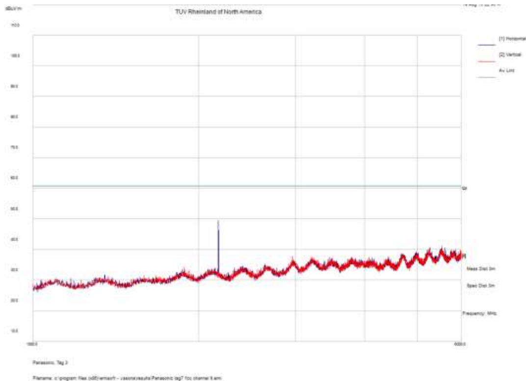
Figure 24: 1-6 GHz, 434.568 MHz
