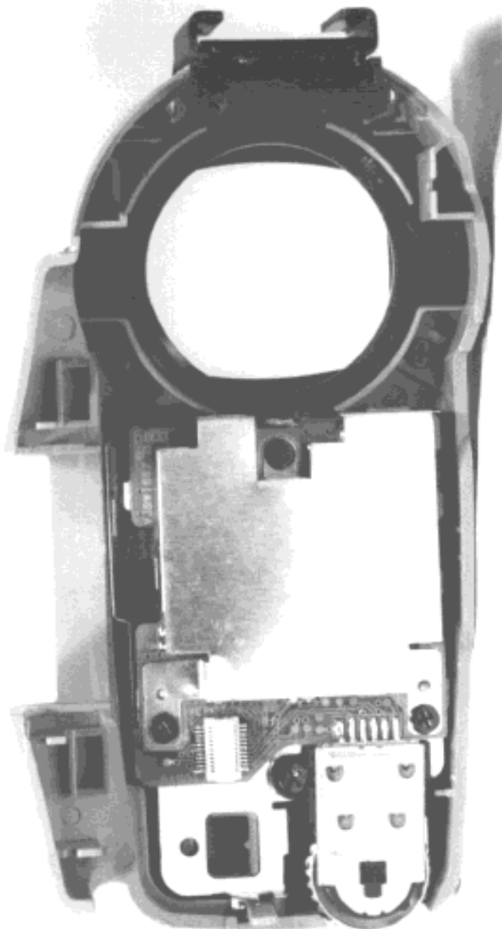
Microphone PCB (BOTTOM VIEW)
