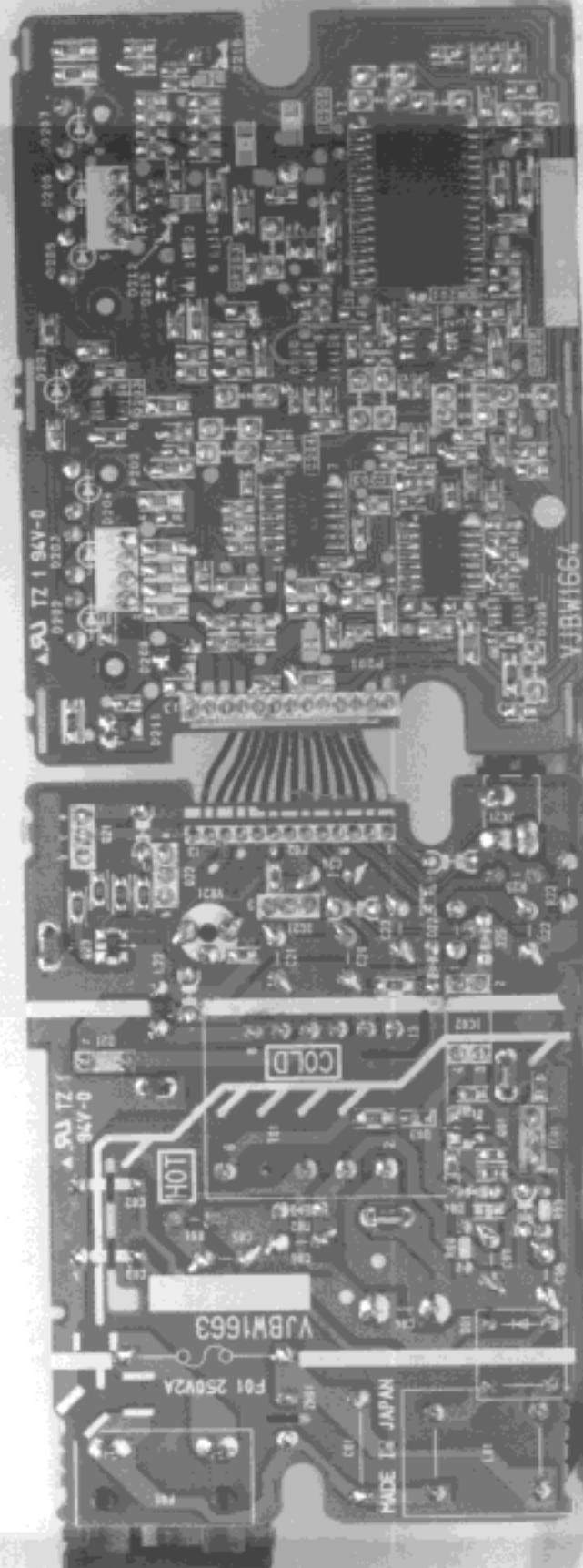
AC Adaptor PCB (BOTTOM VIEW)
