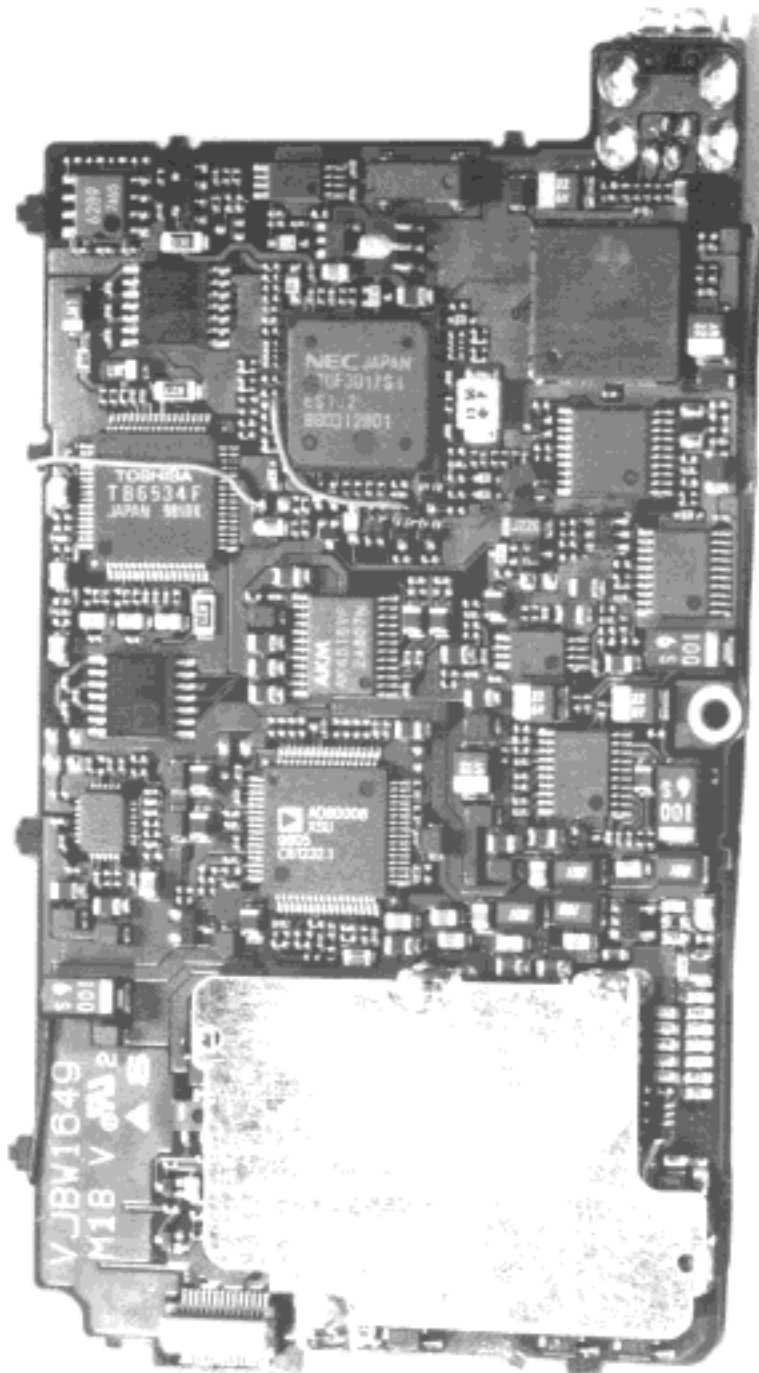
Main PCB (BOTTOM VIEW)
