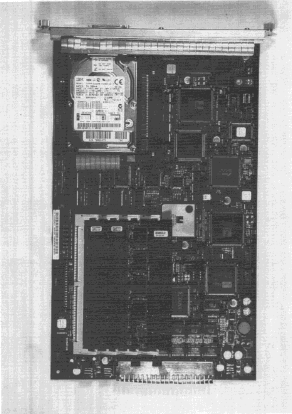
Photo 5 Top view of Printer Main Control Board with Option Hard Disk, Frame and Expansion DIMM option added.
