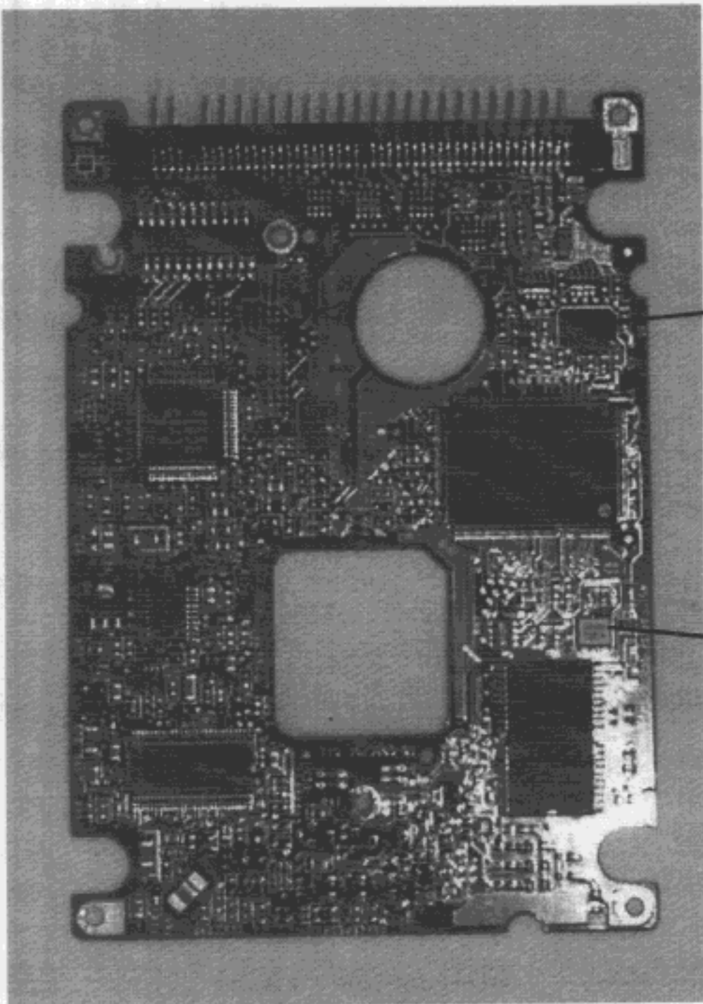
Photo 12 Top view of Option HDD Board.
