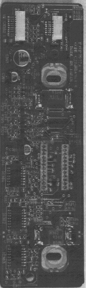
CCD Board
