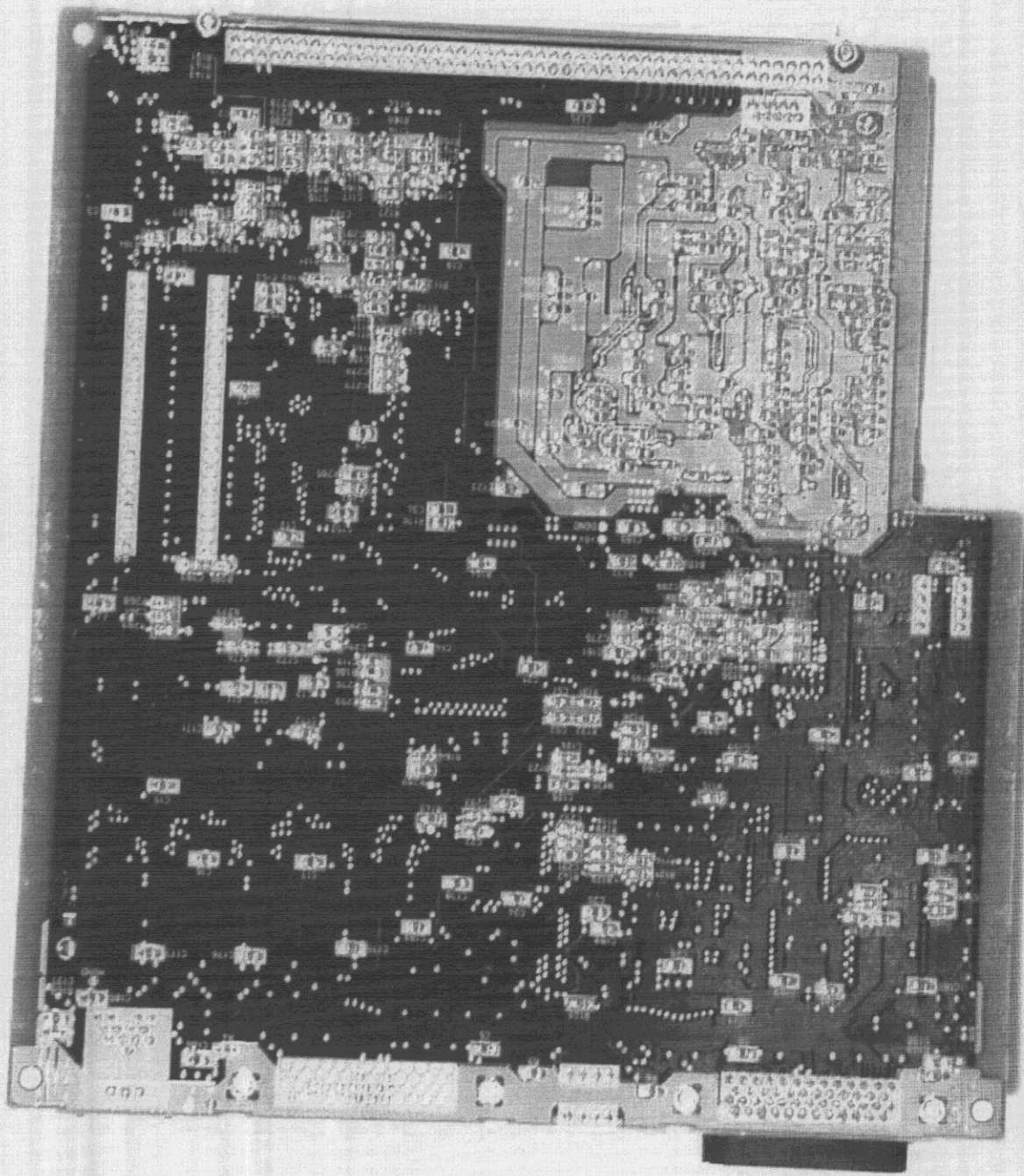
Photo 8 Bottom view of Main Board.
