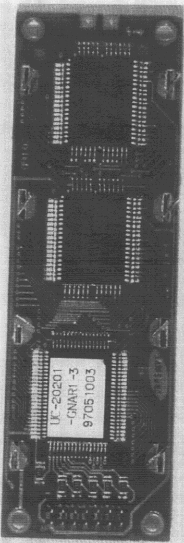
LCD Board
