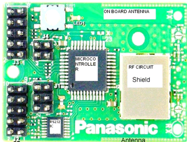
PAN802154 TOP VIEW WITH ALL OPTIONS INCLUDED: LED, TOUCH SWITCH, J1, J2, J3, J4, RS232 IC
