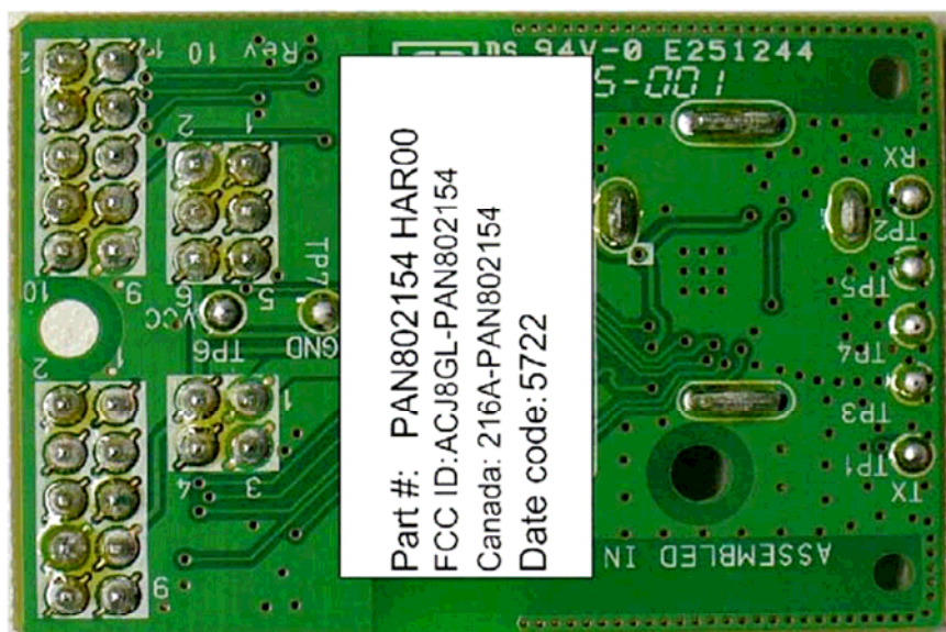
PAN802154 BOTTOM VIEW
