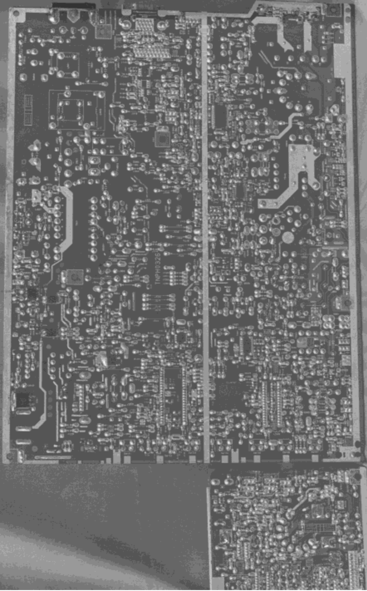
Fig 5. Main & CRT PWB, Foil Side
