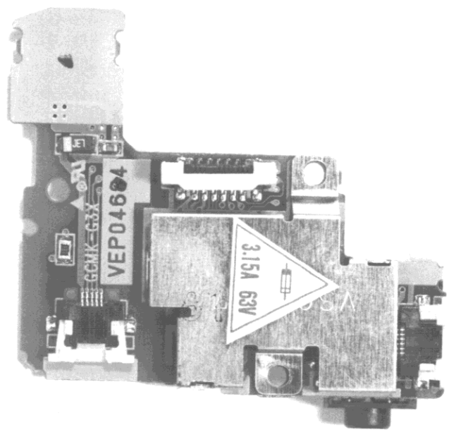
Microphone PCB (TOP VIEW)
