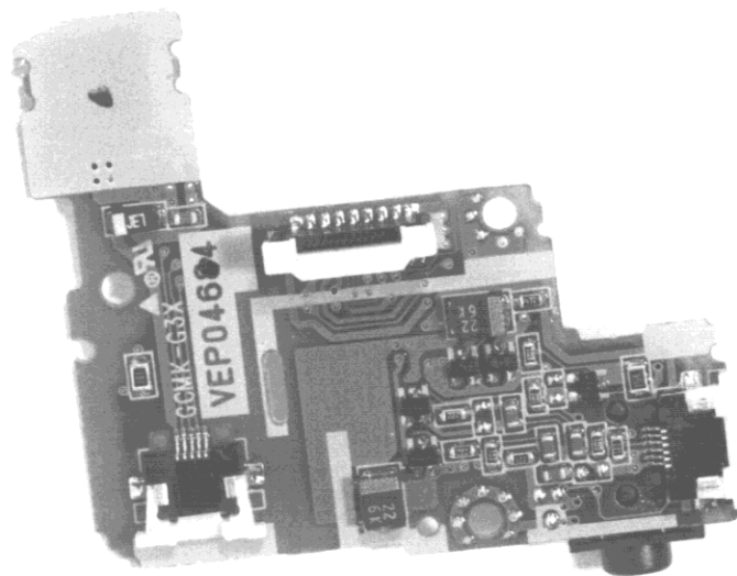
Microphone PCB (TOP VIEW)
