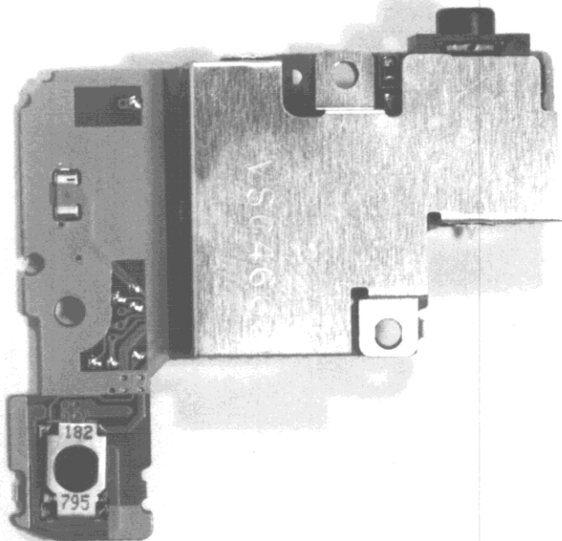
Microphone PCB (BOTTOM VIEW)
